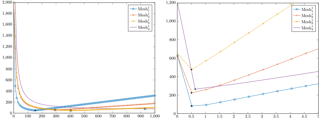
Fig. 14 Test 1, (\text{Mesh}_m^1)_m, m = 1, 2, 3, 4 . Left : optimization of \lambda to obtain an error of order 10^{-5} , with \alpha = 1, \beta = 10^{-1} . Right : optimization of \alpha to obtain an error of order 10^{-5} , with \lambda = 100, \beta = 10^{-1} .
