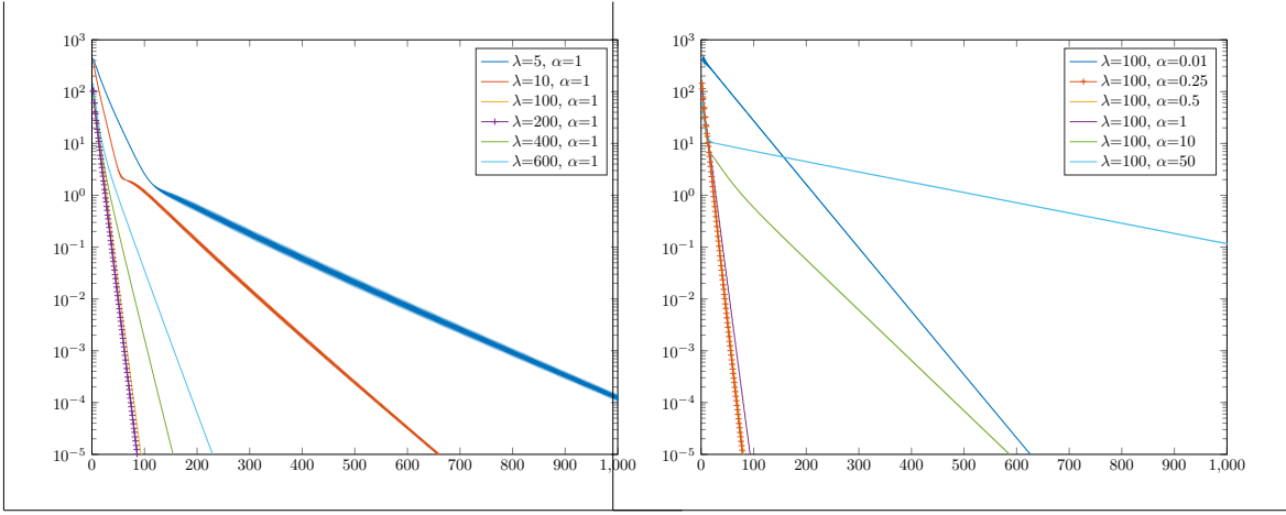
Fig. 11 Test 1, \text{Mesh}_1^1 , first Schwarz algorithm. Left : optimization of \lambda , with \alpha = 1 , \beta = 10^{-2} . Right : optimization of \alpha , with \lambda = 100 , \beta = 10^{-2} .
