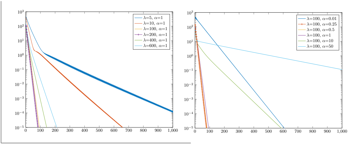
Fig. 12 Test 1, \text{Mesh}_1^1 , second Schwarz algorithm. Left : optimization of \lambda , with \alpha = 1 , \beta = 10^{-2} . Right : optimization of \alpha , with \lambda = 100 , \beta = 10^{-2} .
