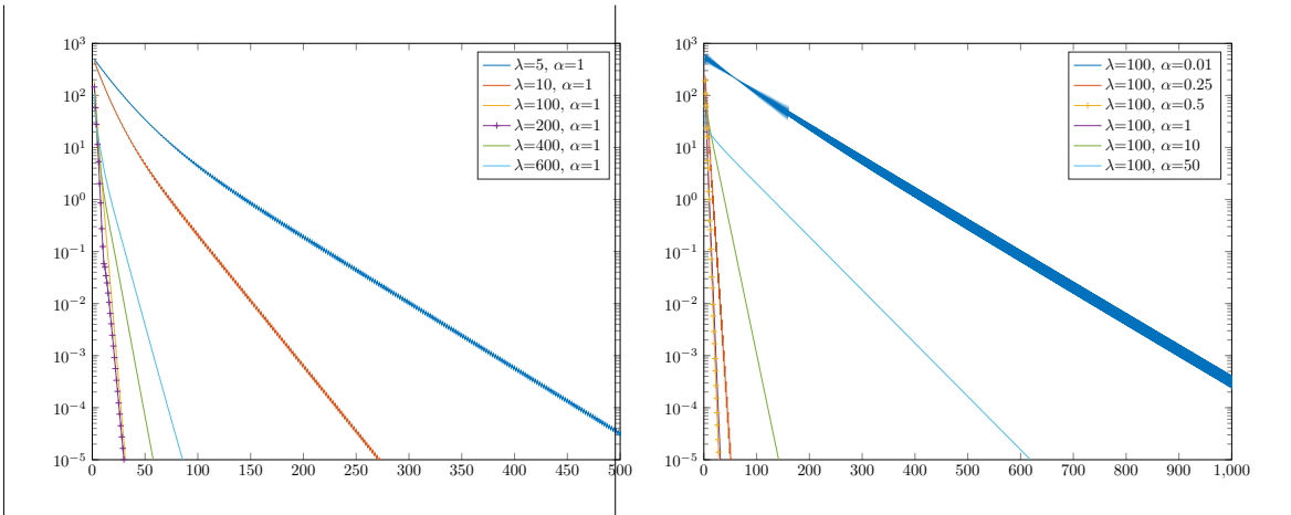
Fig. 13 Test 2, \text{Mesh}_1^2 , first Schwarz algorithm. Left : optimization of \lambda , with \alpha = 1 , \beta = 10^{-2} . Right : optimization of \alpha , with \lambda = 100 , \beta = 10^{-2} .
