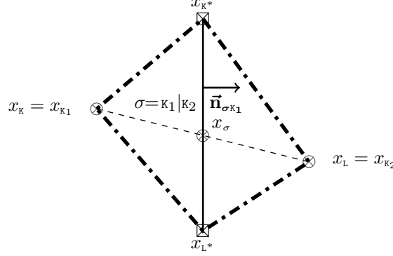
Fig. 6 A diamond \mathfrak{D} , of vertices x_k, x_{k^*}, x_{l^*}, x_l as a union of two semi-diamonds: \mathfrak{D}_1 of vertices x_{k_1}, x_{k_1^*}, x_{\sigma_1}, x_{\sigma_1^*} and \mathfrak{D}_2 of vertices x_{k_2}, x_{k_2^*}, x_{\sigma_2}, x_{\sigma_2^*} . In particular, \sigma_1^* = [x_{k_1}, x_{l^*}] and \sigma_2^* = [x_{l^*}, x_{k_2}] .
