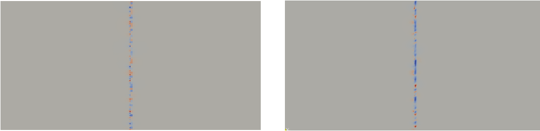
Fig. 9 Error \mathbf{u}_x^1 - \mathbf{u}_x at the 1 st iteration. Left : Primal mesh, \|\mathbf{u}_{\mathcal{M}}^1 - \mathbf{u}_{\mathcal{M}}\|_\infty = 1.9 . Right : Dual mesh, \|\mathbf{u}_{\mathcal{M}^* \cup \partial\mathcal{M}^*}^1 - \mathbf{u}_{\mathcal{M}^* \cup \partial\mathcal{M}^*}\|_\infty = 6.9 .
