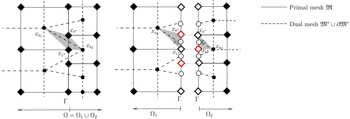
Fig. 4 DDFV meshes.
