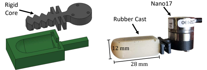
(a) Mold used to shape the FS. (b) The complete FS.
