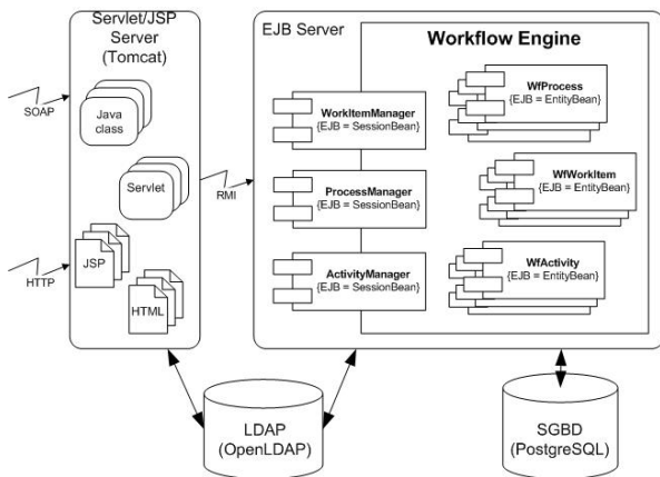
FIG. 1 – Workflow architecture
