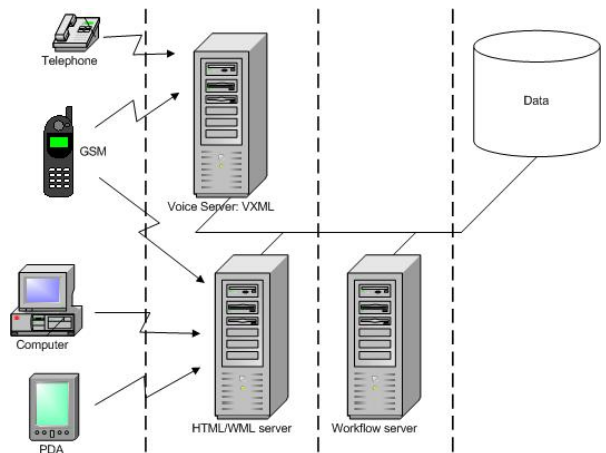
FIG. 2 – Platform architecture
