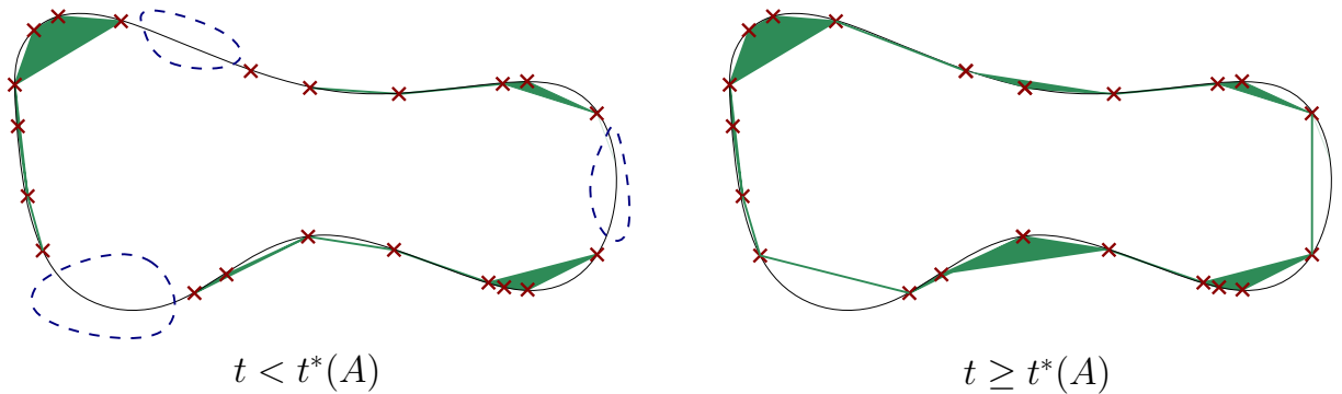
Figure 3 – The t -convex hull of the finite set A (red crosses) is displayed (in green) for two values of t . The black curve represents the (one dimensional) manifold M . On the first display, the value of t is smaller than t^*(A) , as there are regions of the manifold (circled in blue) which are not attained by the projection \pi_M restricted to the t -convex hull. The value of t is larger than t^*(A) on the second display.
