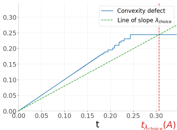
(b) Choice of t - Torus
