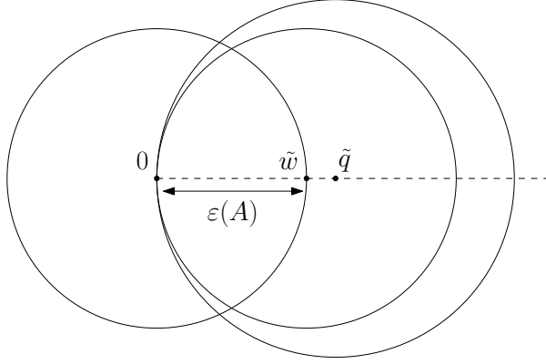
Figure 4 – If |\tilde{q}| > \varepsilon(A) , then the ball \mathcal{B}_{T_0M}(\tilde{q}, |\tilde{q}|) contains a ball of radius \varepsilon(A) centered at a point (here denoted by \tilde{w} ) at distance less than \varepsilon(A) from 0.
