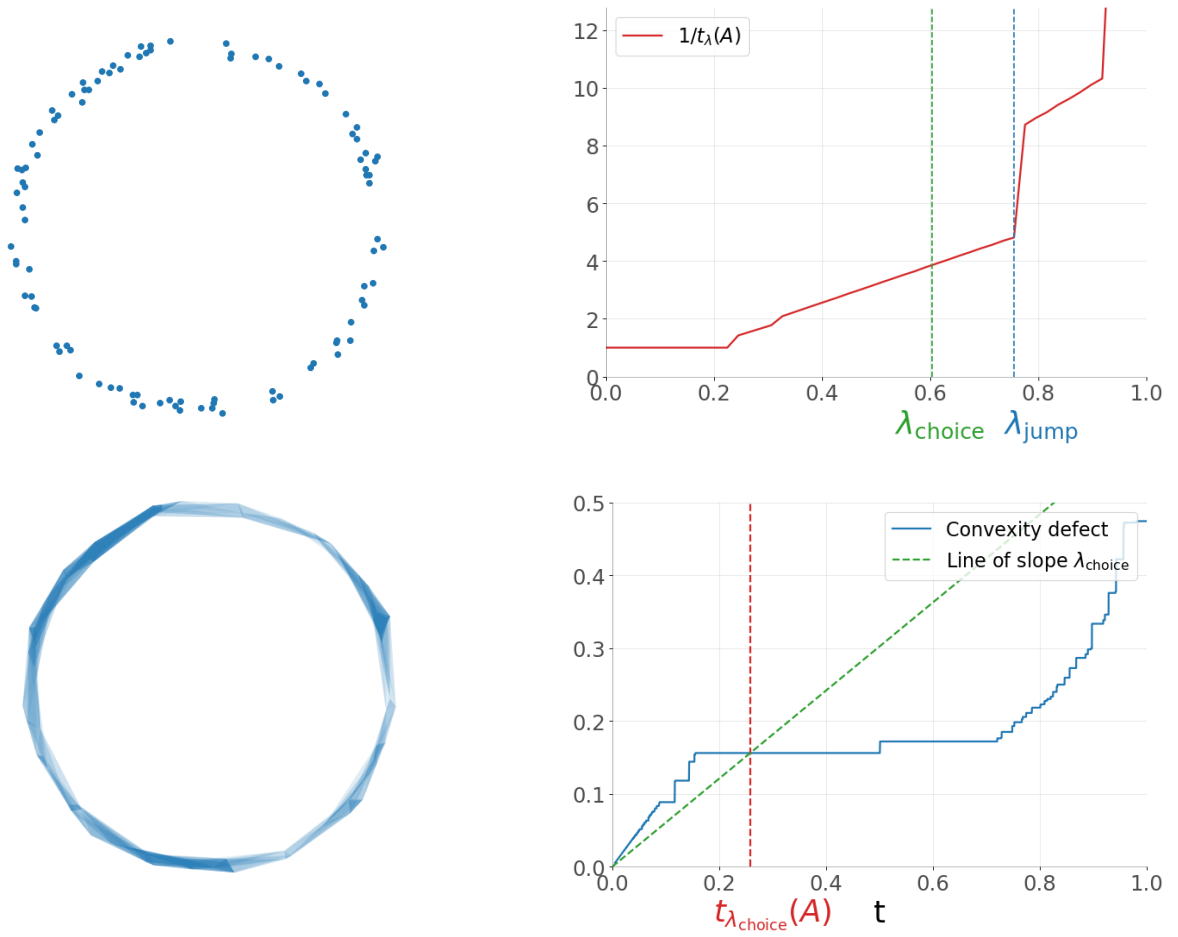
Figure 8 – Top left. Sample \mathcal{X}_n . Top right. The value of \lambda_{\text{choice}}(\mathcal{X}_n) is equal to 0.8\lambda_{\text{jump}}(\mathcal{X}_n) . Bottom left. The set \text{Conv}(t_{\text{sel}}(\mathcal{X}_n), \mathcal{X}_n) . Bottom right. The graph convexity defect function h(\cdot, \mathcal{X}_n) .
