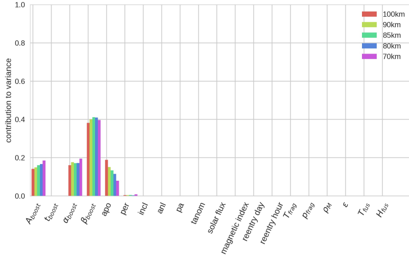
Figure 9: Longitude sensitivity index at 100km, 90km, 85km, 80km, 70km
