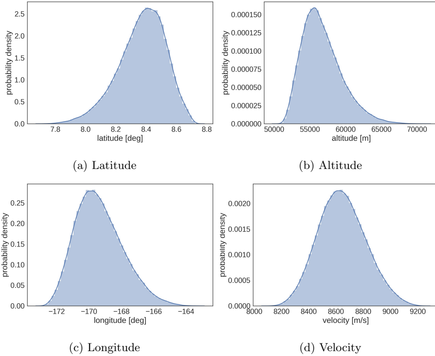
Figure 6: Flight conditions distributions at t_{end}
