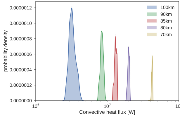
Figure 14: Convective heatflux distributions at 100km, 90km, 85km, 80km, 70km
