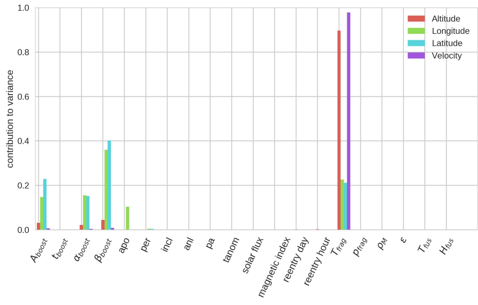
Figure 5: Sensitivity indices at t_{init}
