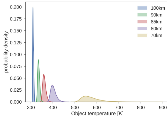
Figure 18: Object temperature distributions at 100km, 90km, 85km, 80km, 70km
