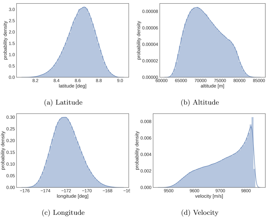
Figure 4: Distributions at t_{init}
