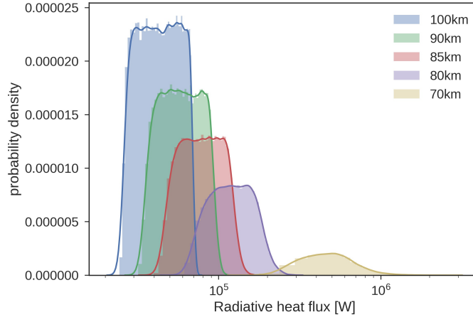
Figure 16: Radiated heatflux distributions at 100km, 90km, 85km, 80km, 70km
