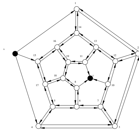
Fig. 11: Dodecahedron
