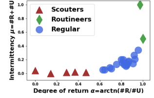
Figure 4: Macaco
