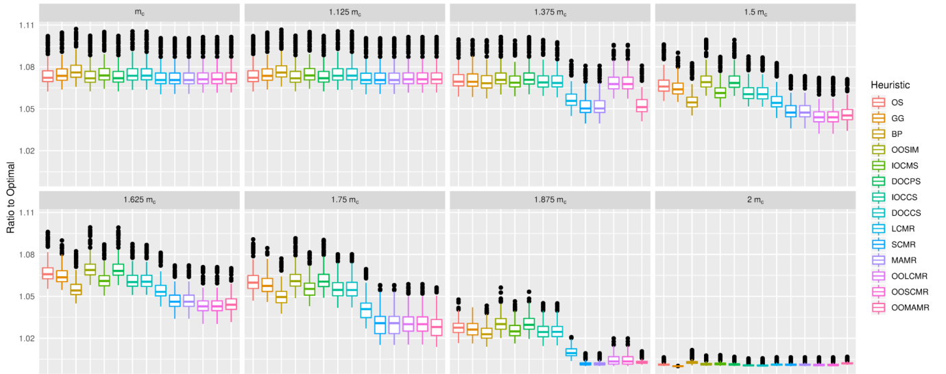
Figure 7: Comparison of different heuristics for HF with m_c = 176KB .
