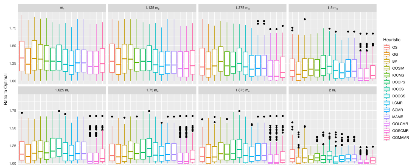
Figure 9: Comparison of different heuristics for CCSD with m_c = 1.8GB .
