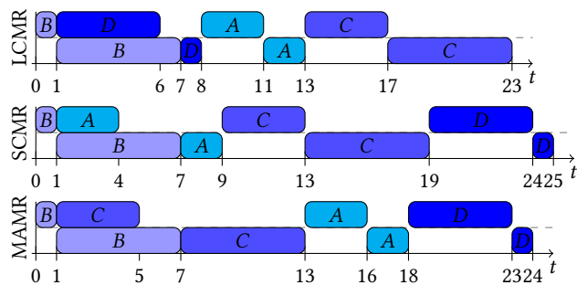
Figure 4: Different dynamic heuristic schedules for a task set of Table 4 with a memory capacity of 6.
