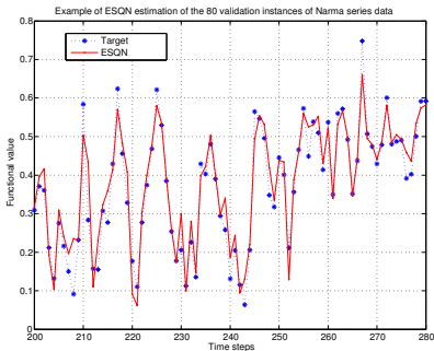
Figure: NARMA validation data set. The reservoir was randomly initialized and it had 80 units.
