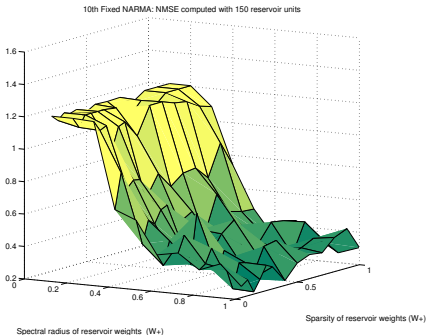
Figure: Simulated dataset. The NMSE according to the spectral radius and the sparsity of the reservoir w^+ .
