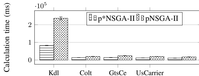
Fig. 14: Calculation time of p*NSGA-II and pNSGA-II
