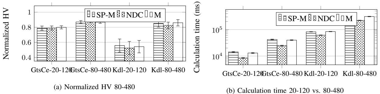
Fig. 17: Performance 20-120 vs. 80-480
