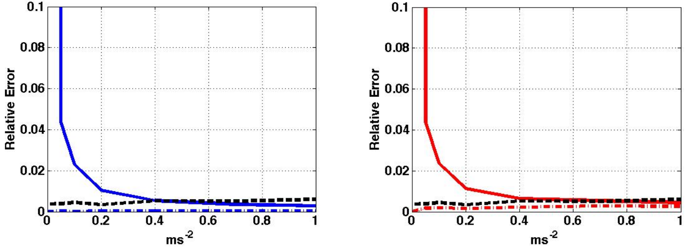
Fig. 1: Results on the \mathcal{S}_1 singularity. The relative error vs \sigma_{a_r} . On the left: the error on the relative position (solid blue), on the relative position up to a scale (dashed blue) and on the relative orientation (dashed black). On the right: the error on the relative speed (solid red), on the relative speed up to a scale (dashed red) and on the relative orientation (dashed black).
