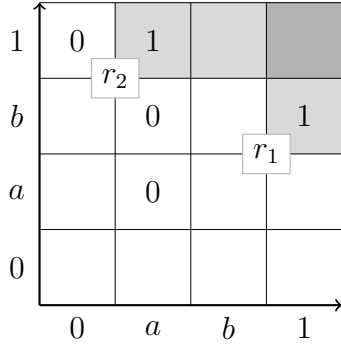
Figure 5: \mathcal{M} and rules of R^- .
