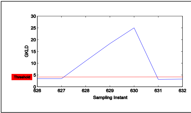
Fig. 11. The jump in the GKLD representing a fault detection.
