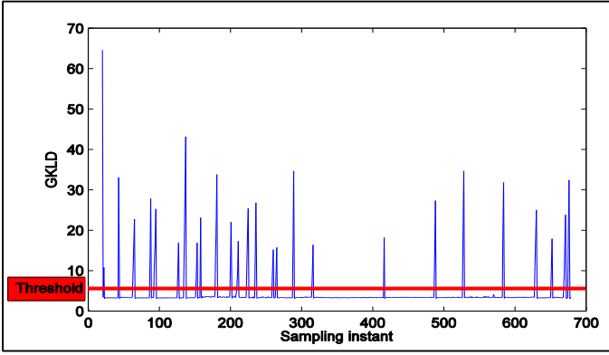
Fig. 10. The GKLD used for fault detection.
