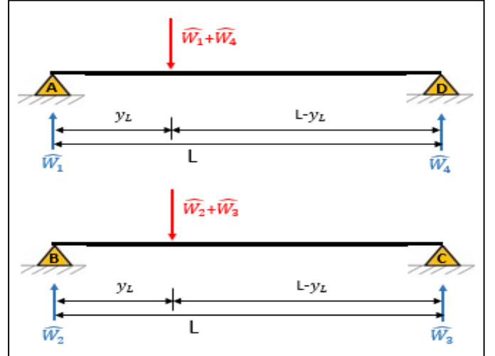
Fig. 3. The weight ( W ) is divided into two parts: ( \widehat{W}_1 + \widehat{W}_4 ) on [AD] (top) and ( \widehat{W}_2 + \widehat{W}_3 ) on [BC] (down).
