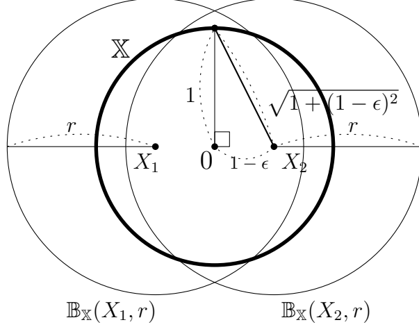
Figure 3: An example in which \mathbb{B}_{\mathbb{X}}(X_1, r) \cup \mathbb{B}_{\mathbb{X}}(X_2, r) is not homotopic equivalent to \check{C}ech_{\mathbb{X}}(\mathcal{X}_n, r) where \mathbb{X} = \{x \in \mathbb{R}^2 : \|x\|_2 = 1\} , X_1 = (-1 + \epsilon, 0) , X_2 = (1 - \epsilon, 0) and r > \sqrt{1 + (1 - \epsilon)^2} , for any \epsilon > 0 .
