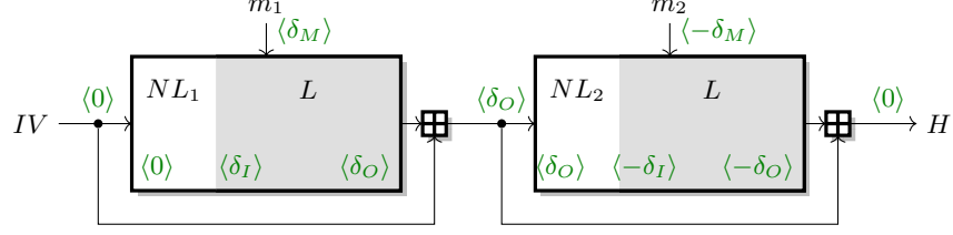
Fig. 1. 2-block collision attack using a linear trail \delta_I \overset{\delta_M}{\rightsquigarrow} \delta_O and two non-linear trails 0 \rightsquigarrow \delta_I and \delta_O \rightsquigarrow -\delta_I . Green values between bracket represent differences in the state.
