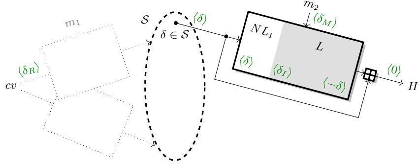
Fig. 2. Single-block chosen-prefix collision attack with a birthday stage. The linear trail \delta_I \rightsquigarrow \delta_O is relaxed to reach a set S of feasible differences.
