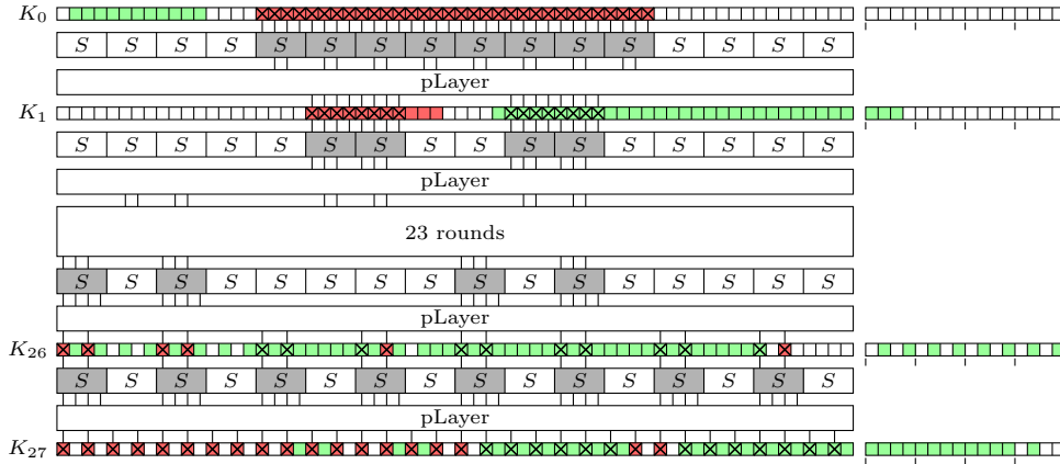
Figure 7: Our attack on 27-round PRESENT using 128 approximations and taking account of the key schedule. All the necessary subkey bits can be deduced from the |k_T|=68 bits which have been highlighted in (dark) red.
