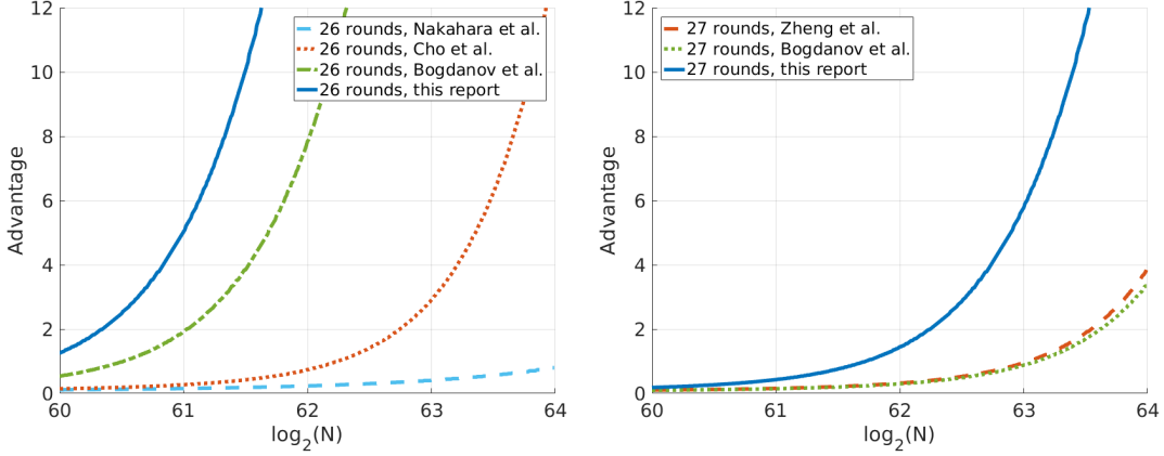
Figure 4: Comparison of the expected advantage (with 0.95 probability) of some known linear attacks on 26 and 27-round PRESENT for a given amount of data (in a DKP scenario).
