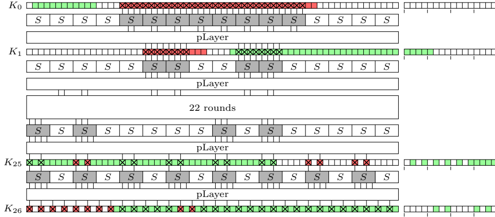
Figure 6: Our attack on 26-round PRESENT using 128 approximations with the analysis of the key schedule. In total there are 96 bits of the subkeys which need to be guessed, which have been indicated by a cross in the figure. However, they can all be deduced from the |k_T|=61 bits of key which have been highlighted in (dark) red. From these bits of key, all the bits in (light) green can be deduced, which includes all the necessary bits for the attack. The 16 bits to the right represent the fraction of the key register which is not used for the current round subkey.
