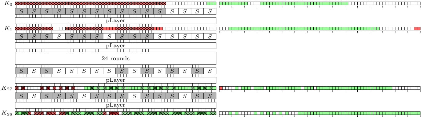
Figure 8: Our attack on 28-round PRESENT-128. In total there are 156 bits of the subkeys which need to be guessed, which have been indicated by a cross. However, if the |k_T|=114 bits of key which have been highlighted in (dark) red are known, then all the bits in (light) green can be deduced, which include all the necessary bits for the attack. The 64 bits to the right represent the half of the key register which is not used for the current round subkey.
