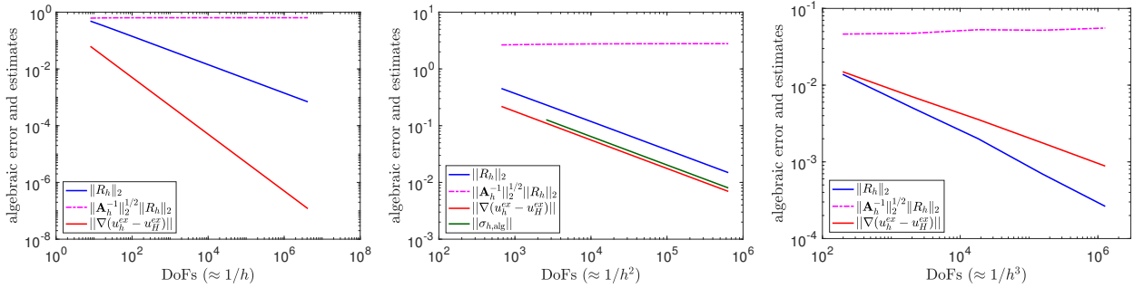
Figure 1: Unit cube problem with u_H^{\text{ex}} as an approximate algebraic solution to u_h^{\text{ex}} . The algebraic error \|\nabla(u_h^{\text{ex}} - u_H^{\text{ex}})\| , the norm \|R_h\|_2 of the associated residual, and the guaranteed upper bound \|\mathbb{A}_h^{-1}\|_2^{1/2} \|R_h\|_2 for the varying mesh size h in one- (left), two- (middle), and three-dimensions (right). For d = 2 , we also plot the guaranteed upper bound \eta_{6.2}^p = \|\sigma_{h,\text{alg}}\| on the algebraic error from (9.9b)
