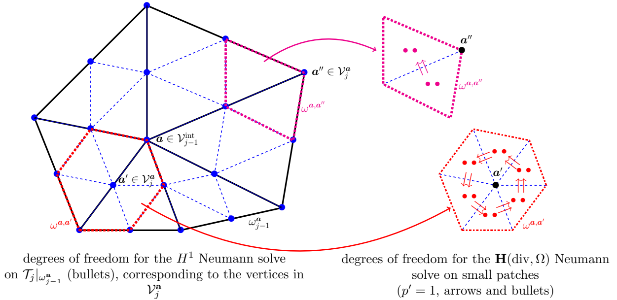
Figure 3: \mathbf{H}(\text{div}, \Omega) -lifting of Construction 6.1 and Construction 6.2 by piecewise affine conforming FEM problem on the large patch subdomain \omega_{j-1}^{\mathbf{a}} and smaller problems posed on small patch subdomains \omega^{\mathbf{a}, \mathbf{a}'} , \mathbf{a}' \in \mathcal{V}_j^{\mathbf{a}}
