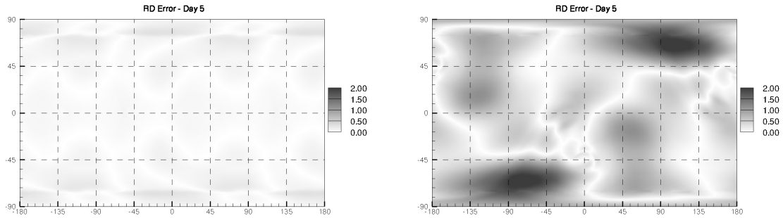
Figure 5: Steady zonal flow. Absolute value of local error on icosahedral grid (forth-level refinement) h_K R^{-1} \approx 0.02 . Black areas correspond to 2m error, white areas to zero error. Left: \alpha = 0 . Right: \alpha = \pi/4 .
