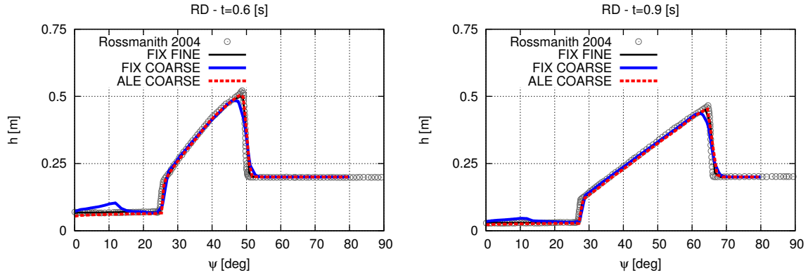
Figure 11: Circular hump on a sphere. Solution along the equator.
