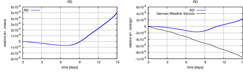
Figure 7: Zonal flow over an isolated mountain. Relative conservation error for mass (left) and energy (right) on gmsh mesh h_K R^{-1} = 0.02 .
