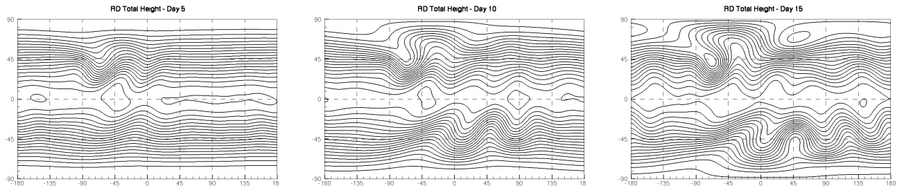
Figure 6: Zonal flow over an isolated mountain. Snapshot of the numerical solution for fixed grid simulation on gmsh mesh h_K R^{-1} = 0.02 at day 5, 10 and 15. Contour levels are from 5050 m to 5950 m in intervals of 50 m.
