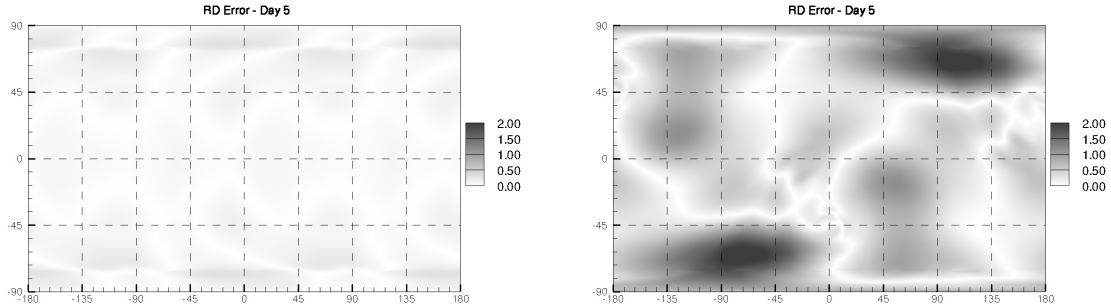
Figure 5: Steady zonal flow. Absolute value of local error on icosahedral grid (fourth-level refinement) h_K R^{-1} \approx 0.02 . Black areas correspond to 2m error, white areas to zero error. Left: \alpha = 0 . Right: \alpha = \pi/4 .
