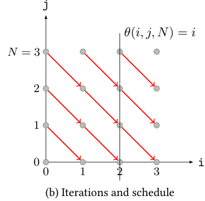
Figure 1. Motivating example
