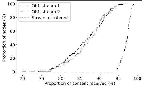
Fig. 8. Cumulative distribution of the proportion of each stream received (1 real interest and 2 obfuscating ones) among nodes (\alpha, K, N) = (0.1, 3, 5) .
