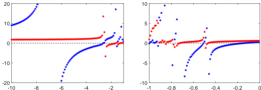
Figure 4.2. Representation of the two eigenvalues of \mathcal{H}(\varepsilon) with respect to \kappa_\varepsilon varying in (-10; -1) (left) and (-1; 0) (right). Here the inclusion Y_i coincides with the rectangle (0.1; 0.9) \times (0.3; 0.7) .
