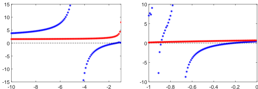
Figure 4.1. Representation of the two eigenvalues of \mathcal{H}(\varepsilon) with respect to \kappa_\varepsilon varying in (-10; -1) (left) and (-1; 0) (right). Here the inclusion Y_i coincides with the interior of the ellipse \{(x = 0.5 + 0.4 \cos \theta, y = 0.5 + 0.2 \cos \theta), \theta \in [0; 2\pi)\} .
