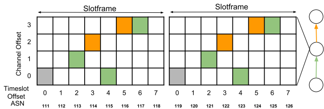
Fig. 2. A 6TiSCH network is synchronized; time is cut into timeslots. Timeslots are organized into slotframes which repeat over time.
