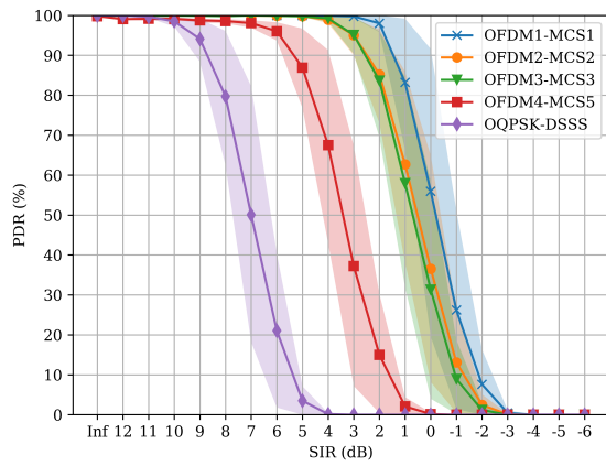
(a) PSDU = 20 bytes
