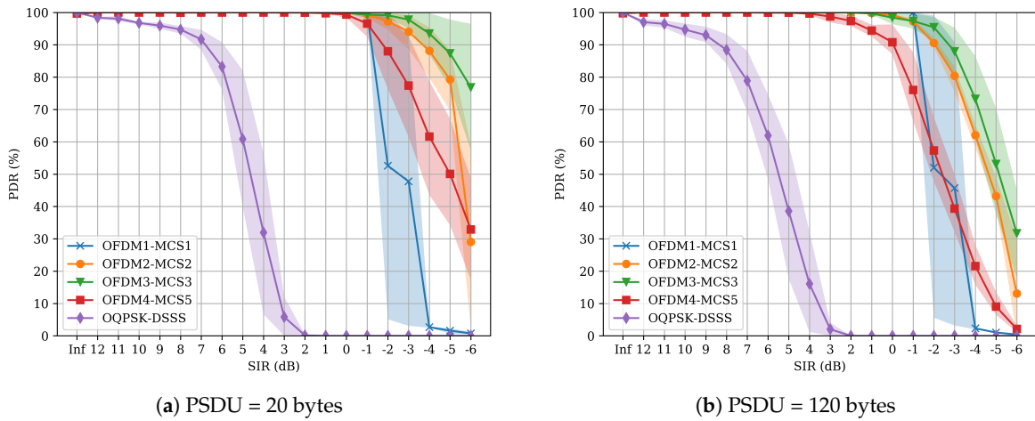
Figure 9. OQPSK-DSSS interference results.
