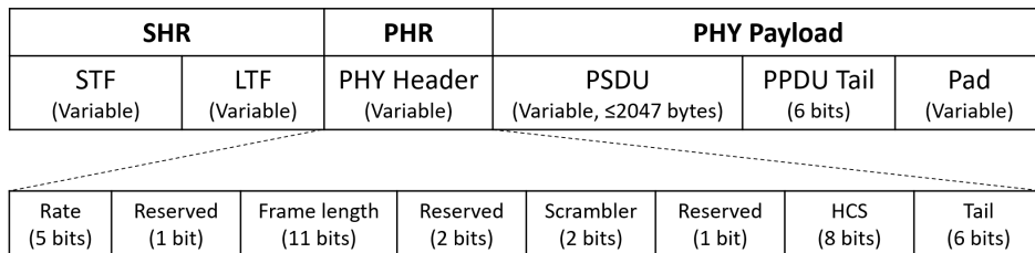
Figure 2. IEEE 802.15.4-2015 SUN-OFDM frame format.
