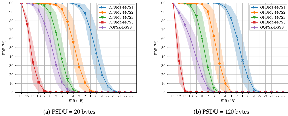
Figure 8. OFDM4-MCS5 interference results.
