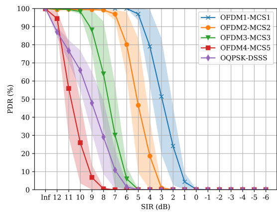
(b) PSDU = 120 bytes
