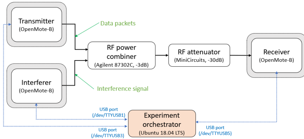
Figure 3. Evaluation setup. Note that the grey box around the transmitter, interferer and receiver devices represents an RF shielding enclosure used to ensure that communication between devices can only occur through the RF coaxial cables.
