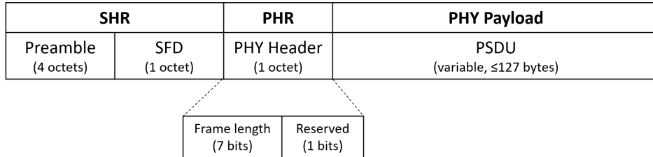
Figure 1. IEEE 802.15.4-2015 OQPSK-DSSS frame format.
