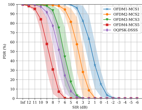
(a) PSDU = 20 bytes
