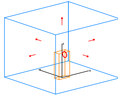
Figure 1. Schematic view of the experimental set-up following the ISO 3746 : 1995 standard. The source (orange) is surrounded by the measurement surface (blue) on which the microphones are positionned (red). The axis are indicated in black and represent unit length. The plane of rotation is represented by the red circle.
