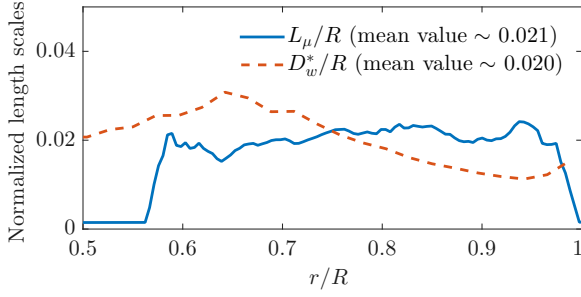
Figure 14. Comparison of length scales representative of turbulence and wake. L_\mu predicted from LBM simulation and D_w^* predicted from the optimization tool. Normalized by tip radius.
