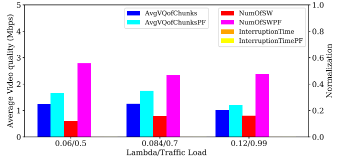
(b) Shadow-Enforcer with minimum-rate variant and PF scheduling with lowest bitrate l_1 = 0.75 \text{ Mbps}
