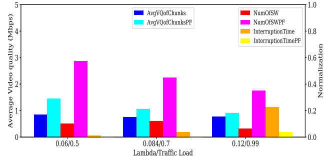
(a) Basic Shadow-Enforcer and PF scheduling with lowest bitrate l_1 = 0.75 \text{ Mbps}
