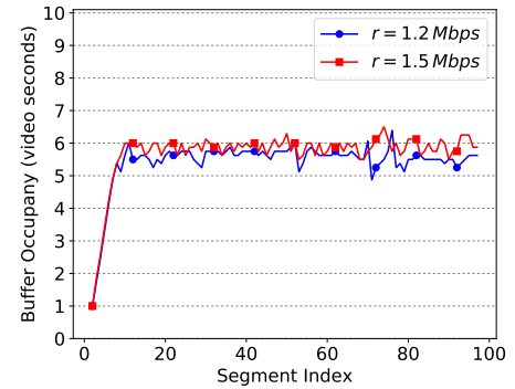
Fig. 2: Evolution of the DASH client's playout buffer level during a 3.2 minute (96 segments of durations 2 seconds each) video.
