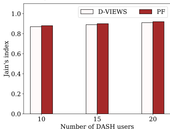
Fig. 15: Jain's index for different number of DASH flows in the systems.
