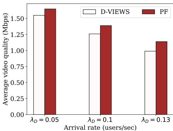
Fig. 11: Average video bitrate for different DASH flow arrival rates.
