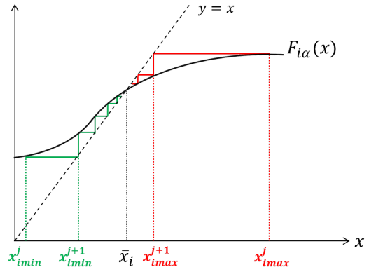
Fig. 2. Illustration of iterations for both sequences: x_{imax}^{j+1} = F_{i\alpha}(x_{imax}^j) (in red) with initial term x_{imax}^1 and x_{imin}^{j+1} = F_{i\alpha}(x_{imin}^j) (in green) with initial term x_{imin}^1 , if F_{i\alpha}(x) has a unique fixed point. The two sequences converge towards \bar{x}_i , with x_{imax}^j decreasing and x_{imin}^j increasing.
