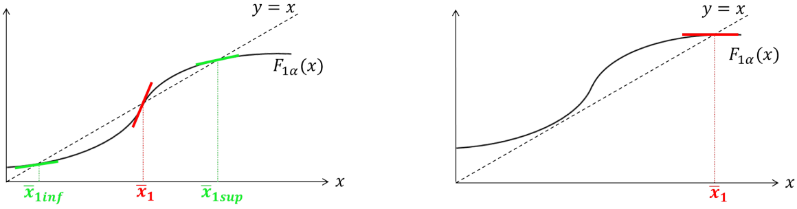
Fig. 4. For both plots, the thick black line is the sigmoid function F_{1\alpha}(x) . The intersections with y = x (represented by the dashed black line) are illustrated. Left: F_{1\alpha}(x) has three fixed points, leading to F_{1\alpha}'(\bar{x}_1) > 1 . Right: F_{1\alpha}(x) has a unique fixed point \bar{x}_1 , leading to F_{1\alpha}'(\bar{x}_1) < 1 .
