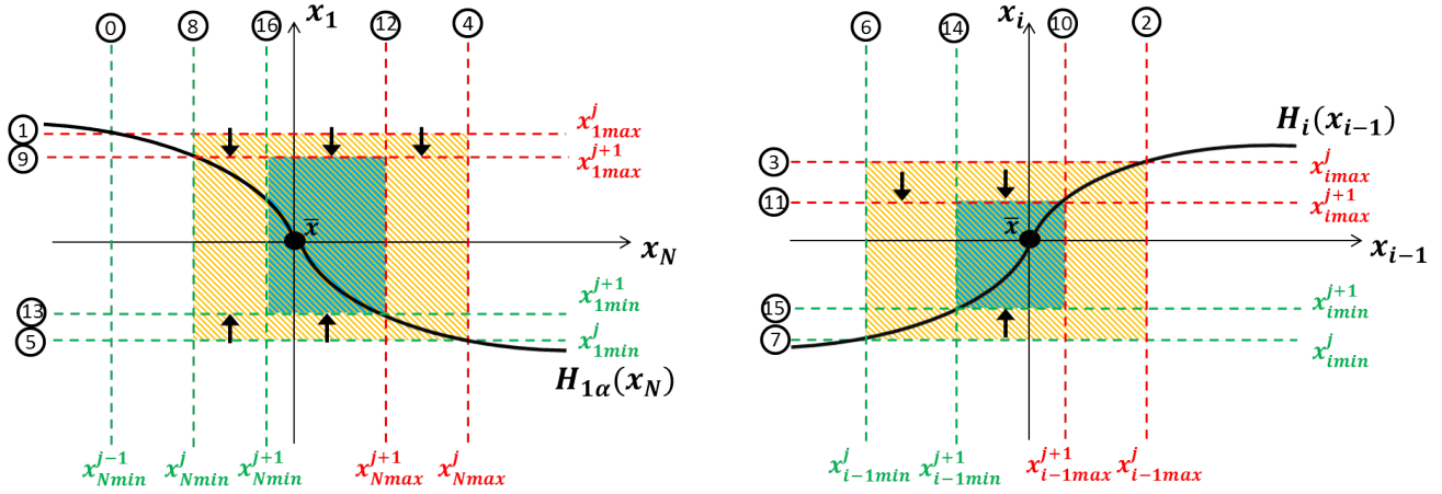
Fig. 3. These two schemes are an illustration of the construction of the successive hyperrectangles. The numbers from 1 to 8 explain the induction steps for the construction of the bounds defining \mathcal{R}^j (represented by orange rectangles), and the numbers from 9 to 16 explain the induction steps for the construction of the bounds defining \mathcal{R}^{j+1} (represented by blue rectangles). The vector field at the borders of \mathcal{R}^j and \mathcal{R}^{j+1} points inward, illustrating the invariant property in Proposition 4. Moreover, by induction, the black arrows show that any trajectory starting in \mathcal{R}^j arrives in finite time in \mathcal{R}^{j+1} , illustrating the repellent property in Proposition 4.
