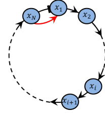
Fig. 1. Graph of the uncontrolled system (1) in black. For the controlled system (3), the graph is the same with the additional red arrow. In this case, the influence of x_N on x_1 is not fixed: it can either activate or inhibit its production.
