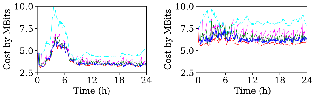
RT n° XXXX Figure 20: Network cost per accepted bandwidth for ta1 (left) and for ta2 (right).
