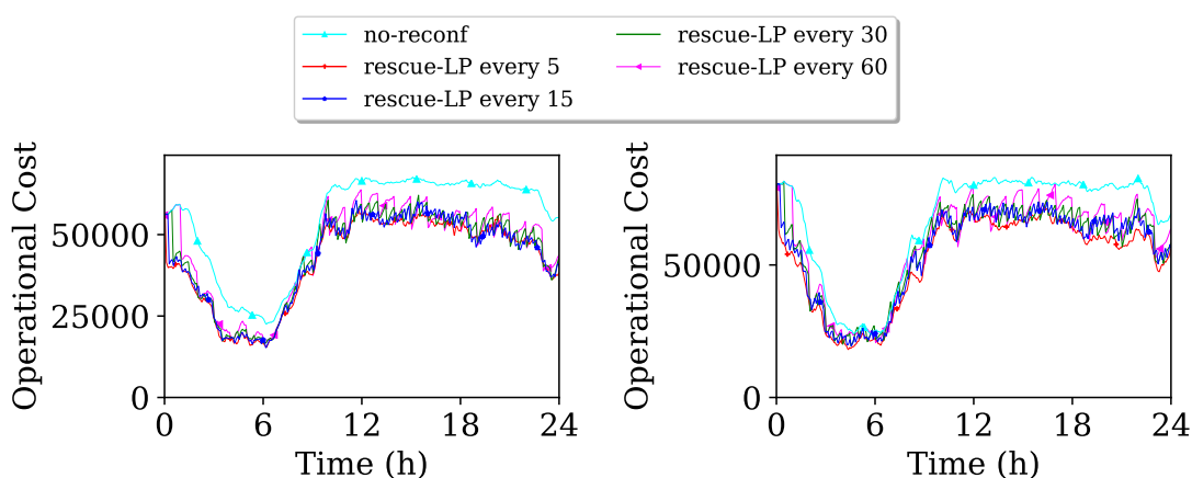
Figure 17: Network cost for ta1 (left) and for ta2 (right).
