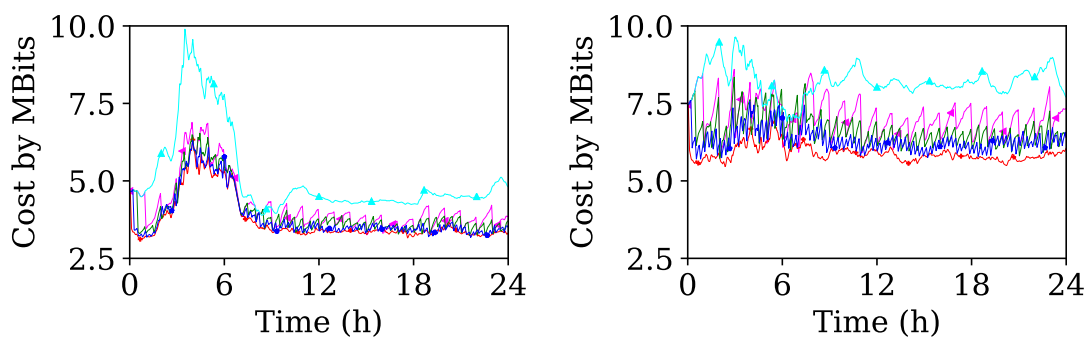
RT n° XXXX Figure 20: Network cost per accepted bandwidth for ta1 (left) and for ta2 (right).
