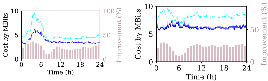
Figure 16: Network cost per accepted bandwidth for ta1 (left) and for ta2 (right).
