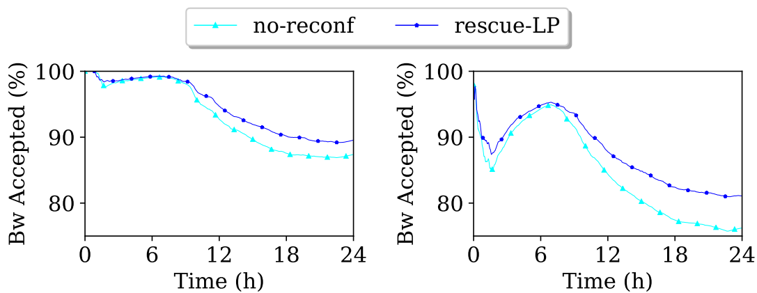
Figure 15: Percentage of Bandwidth accepted for ta1 (left) and for ta2 (right).
