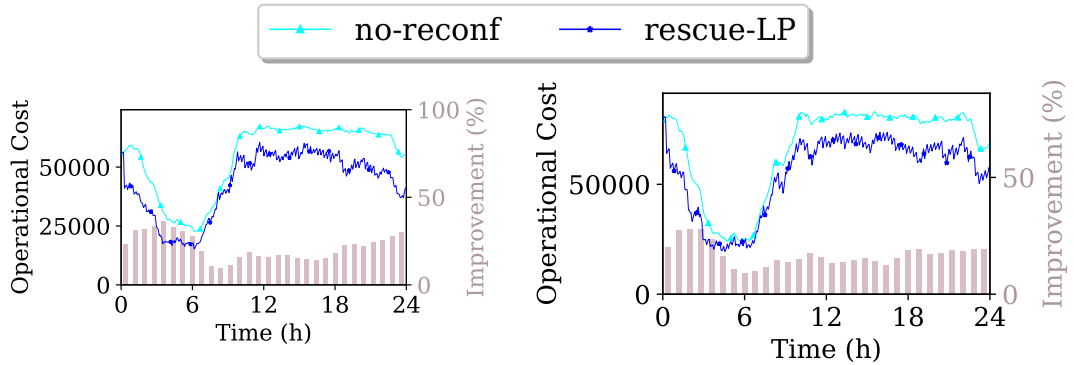
Figure 13: Network cost for \mathbf{ta1} (left) and for \mathbf{ta2} (right).
