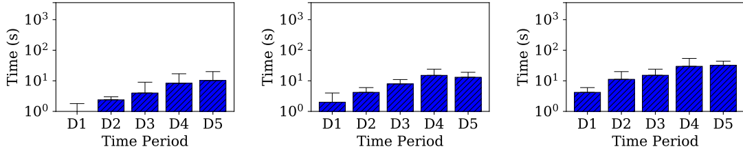
Figure 25: Reconfiguration time with low latencies (left), normal latencies (middle) and high latencies (right) reconfiguration on \mathbf{ta1} .
