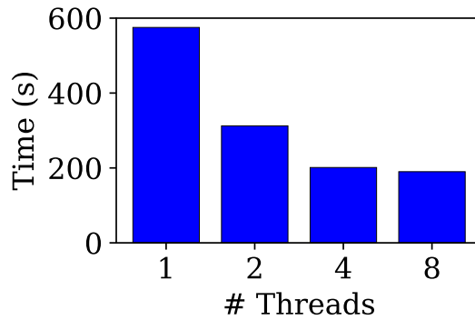
Figure 23: Time to execute the pricing problems according to the number of threads on ta2 with 400 slices.
