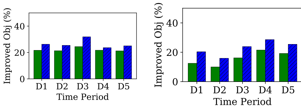
Figure 22: Gains in network cost for ta2 with 300 slices (left) and with 500 slices (right).
