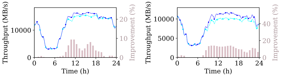
Figure 14: Throughput for \mathbf{ta1} (left) and for \mathbf{ta2} (right).
