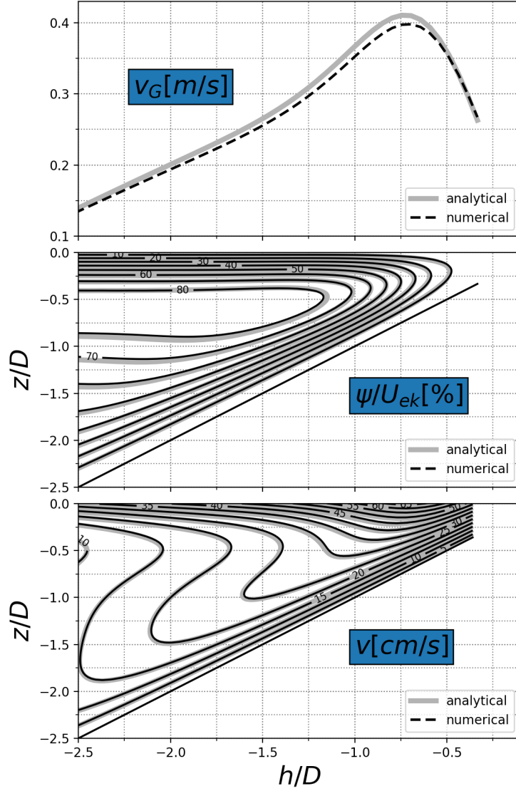
Figure 5: Comparison of the exact analytical and unpenalized numerical solutions using terrain-following \sigma -coordinates for the upwelling test case after 20 days. The horizontal axis gives the distance from the shore in terms of the local normalized depth ( h/D = -2.5 corresponds to x \approx 154 km). Top: the alongshore geostrophic current v_G . Middle: the cross-shore streamfunction \phi normalized by the Ekman transport U_{EK} = |\tau_y/\rho_0 f| . Bottom: the total alongshore velocity v .
