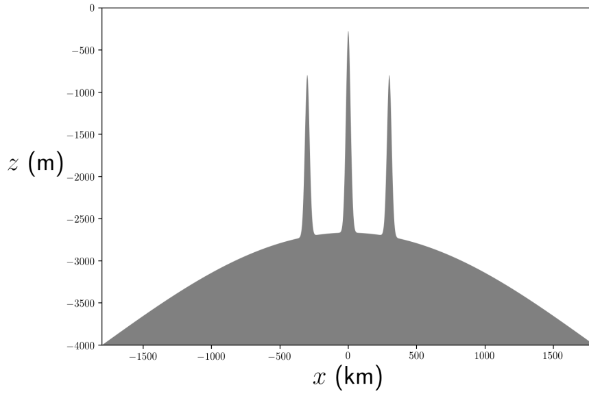
Figure 9: Idealized bathymetry for the internal tide test case.
