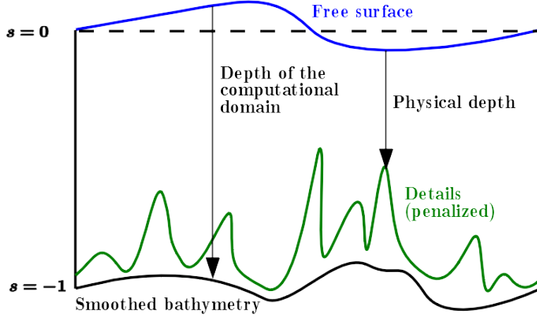
Figure 1: Smoothed bathymetry profile defining the generalized coordinate system (black) and mask defining small scale details (green). The computational domain extends from the surface s(x, t) = 0 to the smoothed bathymetry s(x, t) = -1 . The region between the green and black curves is penalized, with porosity \phi = \alpha \ll 1 .
