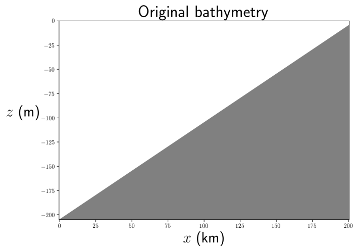
Figure 4: Exact linear bathymetry for the upwelling test case.
