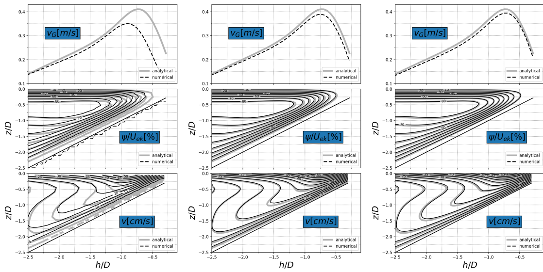
Figure 7: Results obtained for penalized regions of depths h_{\min} = 205 m, 50 m and 10 m (left to right) for the upwelling test cases. The horizontal axis gives the distance from the shore in terms of the local normalized depth ( h/D = -2.5 corresponds to x \approx 154 km). In all cases \epsilon = 4\Delta t and \alpha = 0.01 . As expected, the numerical penalized results converge to the analytical results as the depth of the penalized region decreases (see also table 1).
