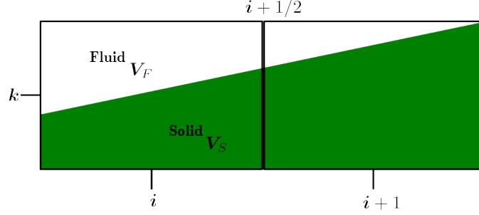
Figure 2: Boundary cells of intermediate porosity \alpha < \phi_{ik} < 1 . The porosity of the cell \phi_{ik} = (V_F + \alpha V_S)/(V_F + V_S) . The green region is the penalized solid.
