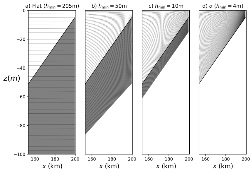
Figure 6: Penalized part of the domain (in grey) and associated vertical levels for three different depths h_{min} of the penalized region, together with the terrain-following \sigma -coordinate case (rightmost figure). Only the first 100 m below the surface is shown. Note that there are vertical levels in the penalized part of the solid region. In the leftmost figure the entire solid region of Fig. 4 is penalized, while the rightmost figure has no penalization ( \sigma -coordinates).
