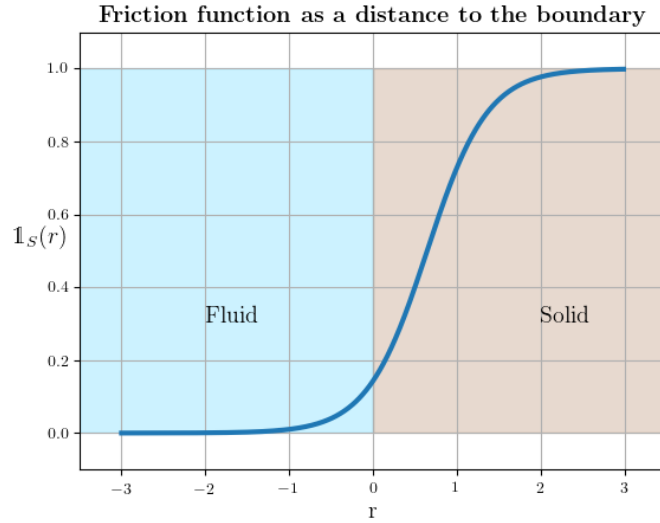
Figure 3: Function \mathbb{1}_S(r) used to smooth the porosity and permeability at the fluid–solid interface in the vicinity of topographical features.
