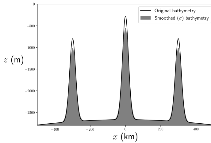
Figure 10: Reference and smoothed (coarse resolution) bathymetries for the internal tide test case.
