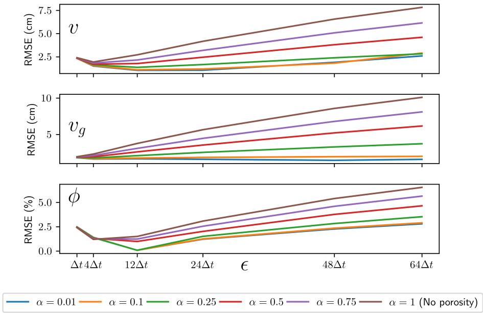
Figure 8: Sensitivity of the numerical solutions (root mean square errors) to the choice penalization permeability \epsilon and porosity \alpha coefficients in the upwelling test case with h_{\min} = 50 m.
