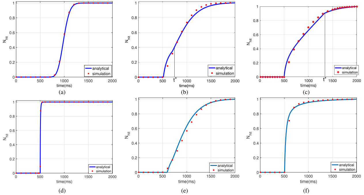
Fig. 2. Comparison of simulation and analytical results for cumulative axial molecule distribution, N_{\text{hit}}(t|d_0, d, x_r) for D = 100 \times 10^{-12} \mu\text{m/s}^2 , x_r = 5\text{mm} , v_m = 10\text{mm/s} and different d values which indicate different Pe regions. (a) d = 5 \mu\text{m} , d_0 = 0 , Pe = 250 , P_c = 4000 . (b) d = 15 \mu\text{m} , d_0 = 0 , Pe = 750 , P_c = 1333 , t^* = 3/4\text{s} . (c) d = 20 \mu\text{m} , d_0 = 0 , Pe = 1000 , P_c = 1000 , t^* = 4/3\text{s} . (d) d = 100 \mu\text{m} , d_0 = 0 , Pe = 5000 , P_c = 200 . (e) d = 15 \mu\text{m} , d_0 = 0.5d , Pe = 750 , P_c = 1333 . (f) d = 40 \mu\text{m} , d_0 = 0.25d , Pe = 2000 , P_c = 500 .
