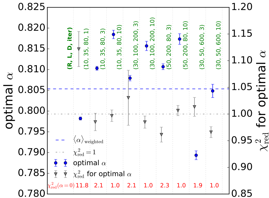
Figure 10: Blue datapoints are the optimal value of \alpha for different input parameters, estimated from the IS-DCD as described in the text. The grey triangles indicate the value of \chi^2_{\text{red}} obtained with this choice of \alpha . We also list the values of \chi^2_{\text{red}} for a simulation in which \alpha = 0 at the bottom of the plot. The average \langle \alpha \rangle is weighted with the square of the individual standard deviations. The values (R, L, D, \text{iter}) are given in units of (\mu\text{m}, \mu\text{m}, \mu\text{m}^2/\text{s}, 10^2) .
