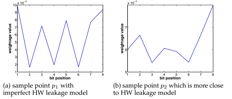
Fig. 7: Sample points with perfect and imperfect HW leakage model
