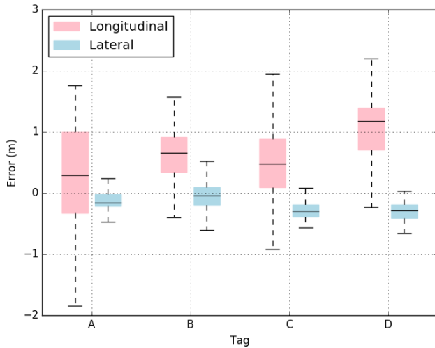
Fig. 8: Box plot of longitudinal and lateral position errors at 4 respective tags using the proposed localization approach for total test runs of 35 km.
