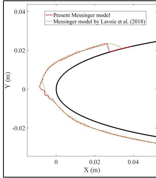
Figure 7: Comparison between the ice accretion of the present model and the literature
