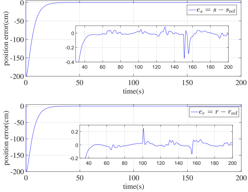
Figure 3: Point stabilization simulation Test-Q position error result
