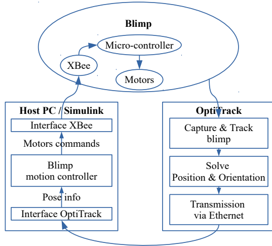
Figure 11: Scheme of Optitrack-enhanced blimp control system
