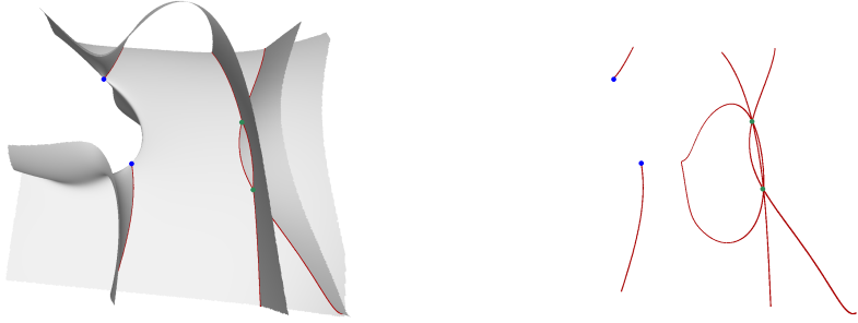
Fig. 2: Left: Singular surface \Omega , projection in \mathbb{R}^3 of the smooth 2-manifold \mathcal{M} of \mathbb{R}^4 defined by Equations (9). Right: Singular curve of \Omega with cross-caps (blue) and triple points (green).
