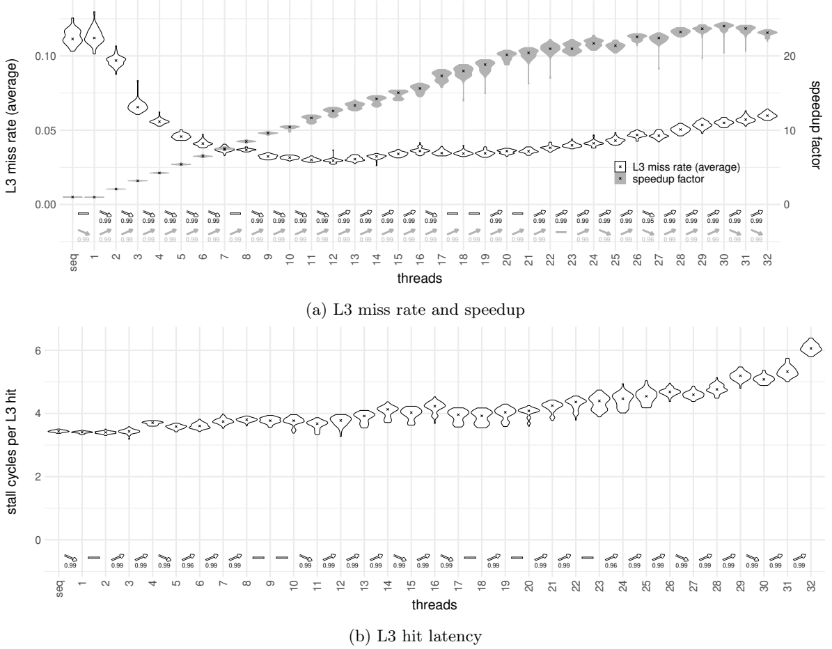
Figure 9: Storage resource conflicts - (simple, ICC, float, interleaved, balanced)
