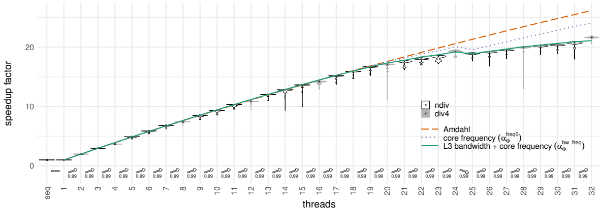
Figure 11: Scalability models - (MKL, ICC, float, interleaved, balanced)
