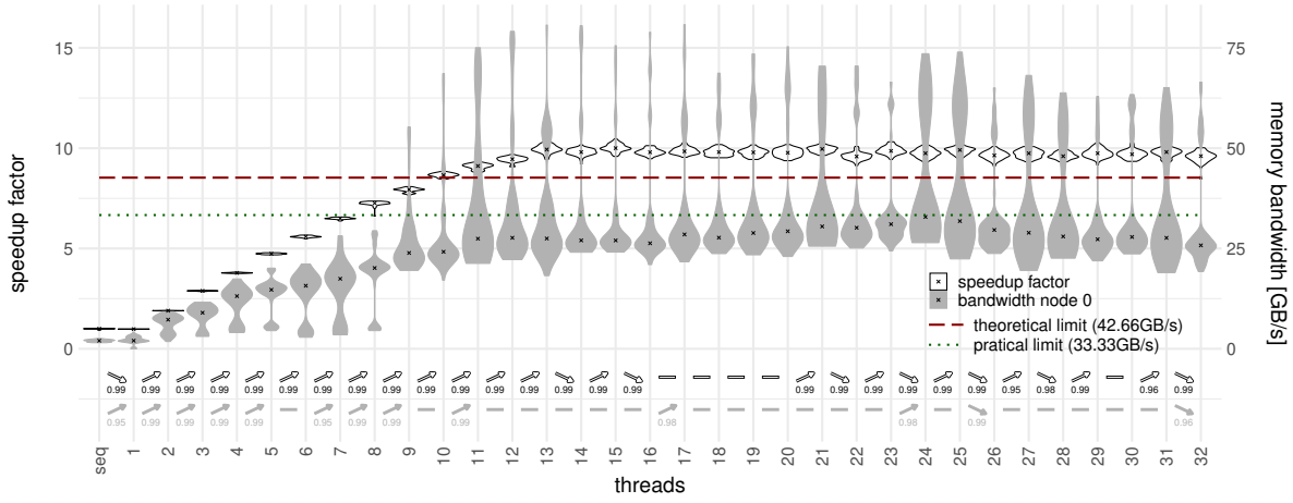
(a) speedup and used bandwidth
