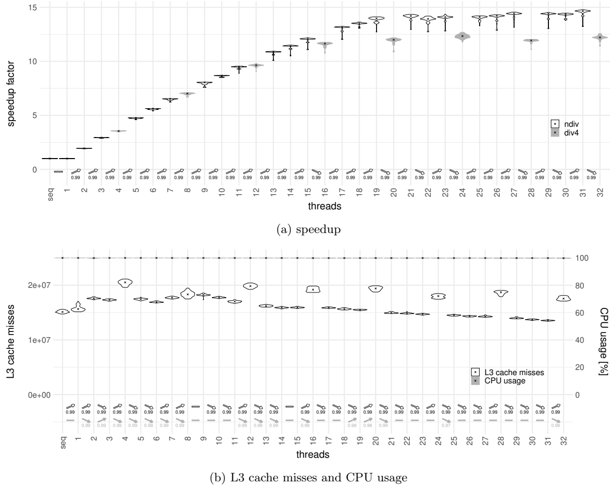
Figure 6: Thread count as implicit input - (MKL, ICC, float, bind, spread)
