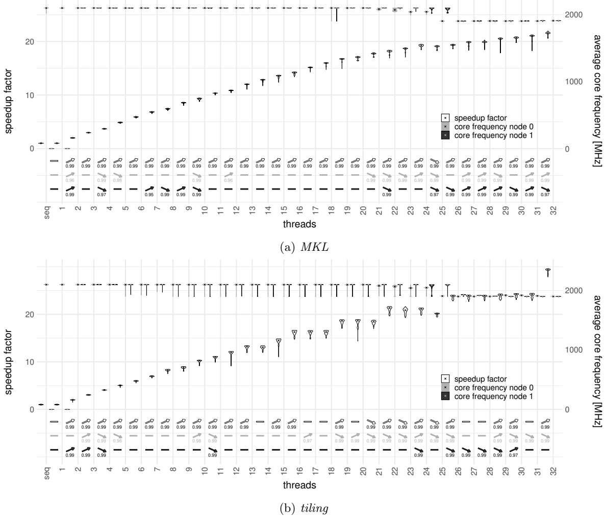
Figure 10: Shared power/temperature budget - (*, Clang, float, interleaved, balanced)
