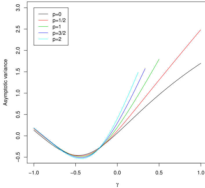
Figure 1: Graphes of \gamma \mapsto \ln \theta(p; \gamma) under the constraint p\gamma < 1 (top panel) and \gamma \mapsto \ln(\gamma^2 + 4\mathcal{V}(p; \gamma)) under the constraint p\gamma < 1/2 (bottom panel) for \gamma \in [-1, 1] , p \in \{0, 1/2, 1, 3/2, 2\} . See Proposition 4 for the definition of \theta(p; \gamma) and Theorem 1 for the definition of \mathcal{V}(p; \gamma) .
