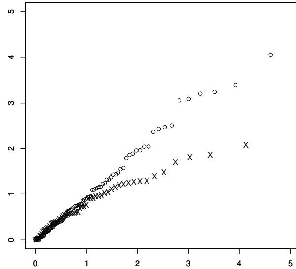
Figure 8: Real data. QQ-plots obtained for years 1980 ( \times \times \times ) and 1985 ( \circ \circ \circ ).
