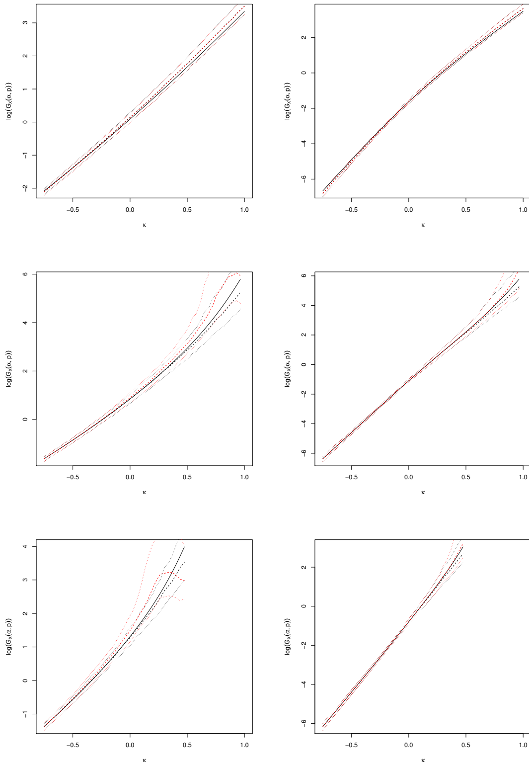
Figure 5: Simulated data, intermediate case with n = 5000 . The continuous line is the graph of the function \kappa \mapsto \ln G_X(\alpha_n; p) . The dashed lines represent the median of the logarithm of the N realizations of the direct (black) and indirect (red) estimators. Dotted lines are the corresponding empirical quantiles of levels 5% and 95%. Top: p = 0 , center: p = 1 , bottom: p = 2 . Left: c = 1/2 , right: c = 2 .
