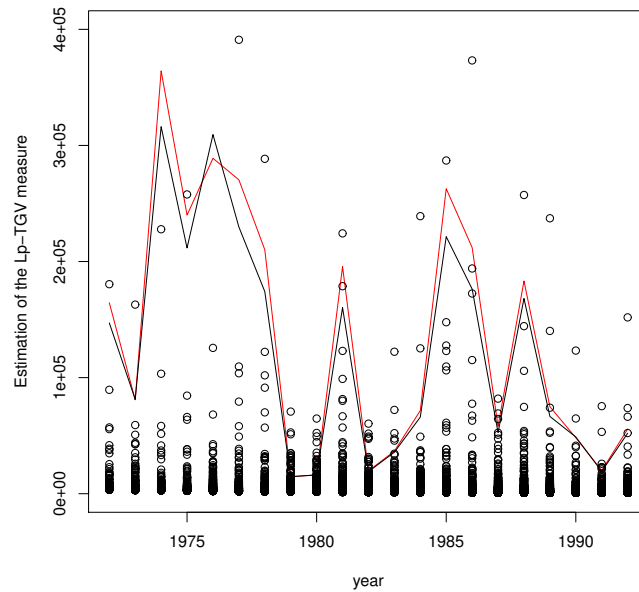
Figure 9: Real data. Estimation of the BC_p -TGV measure for the Norwegian fire losses data set as a function of the year along with the values of the fire losses ( \circ \circ \circ ). In black, the direct extrapolated estimator; in red, the indirect extrapolated estimator. Continuous lines are used for the visualisation sake.
