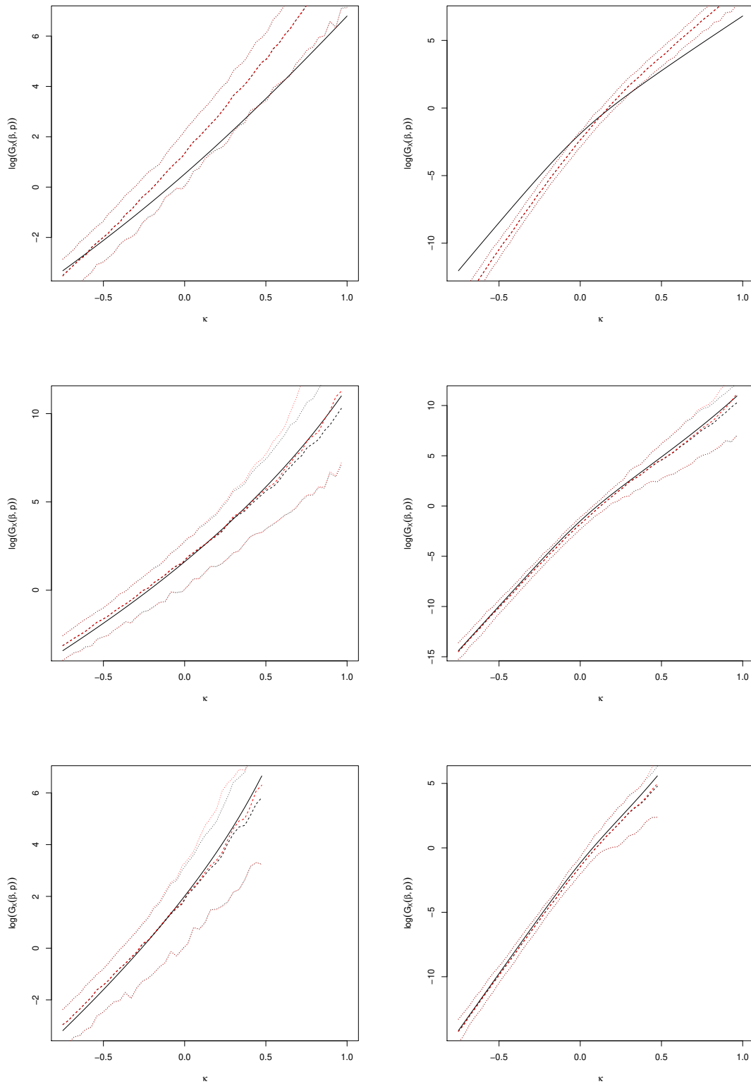
Figure 7: Simulated data, extreme case with n = 5000 . The continuous line is the graph of the function \kappa \mapsto \ln G_X(\alpha_n; p) . The dashed lines represent the median of the logarithm of the N realizations of the direct (black) and indirect (red) extrapolated estimators. Dotted lines are the corresponding empirical quantiles of levels 5% and 95%. Top: p = 0 , center: p = 1 , bottom: p = 2 . Left: c = 1/2 , right: c = 2 .
