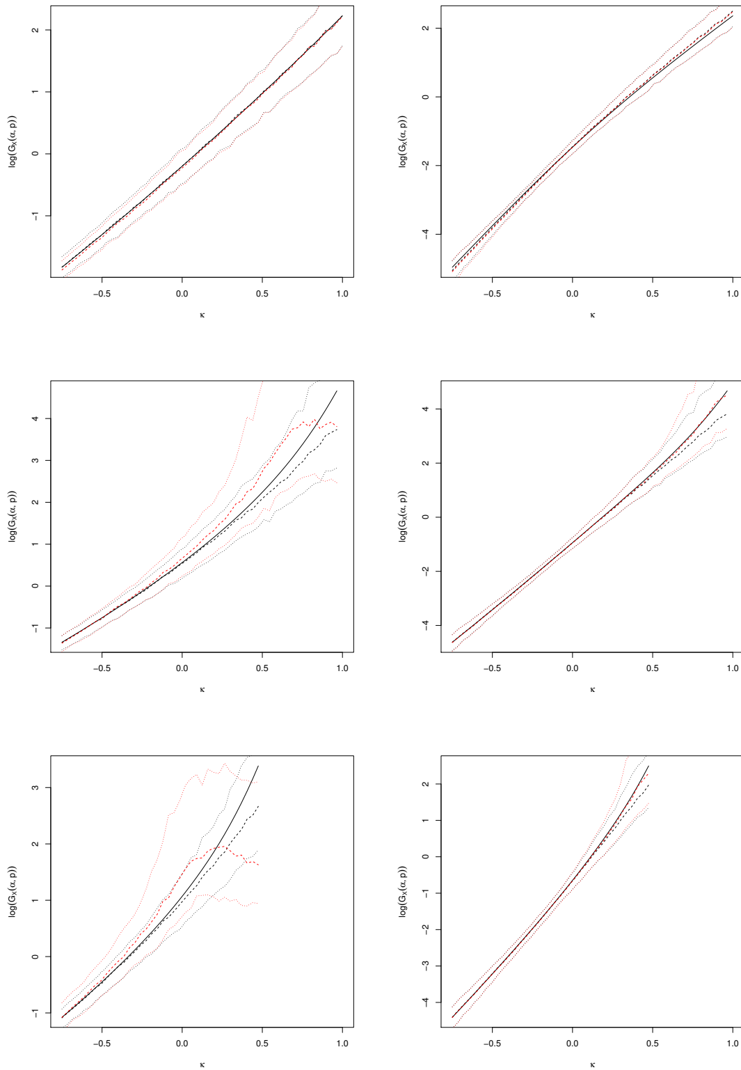
Figure 4: Simulated data, intermediate case with n = 500 . The continuous line is the graph of the function \kappa \mapsto \ln G_X(\alpha_n; p) . The dashed lines represent the median of the logarithm of the N realizations of the direct (black) and indirect (red) estimators. Dotted lines are the corresponding empirical quantiles of levels 5% and 95%. Top: p = 0 , center: p = 1 , bottom: p = 2 . Left: c = 1/2 , right: c = 2 .
