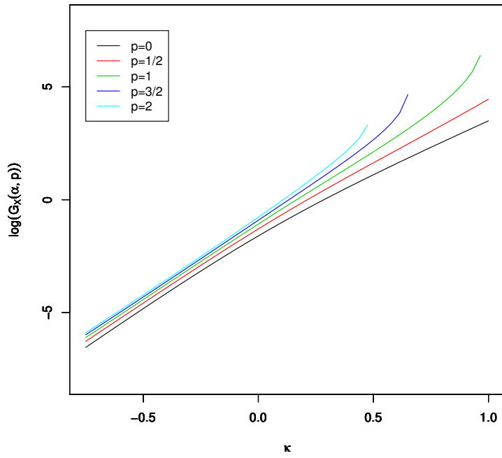
Figure 3: Graph of \ln G_X(\alpha; p) as a function of \kappa \in [-3/4, 1] for the distribution defined in (13) with p \in \{0, 1/2, 1, 3/2, 2\} , \alpha = 0.04 , c = 1/2 (top panel) and c = 2 (bottom panel).
