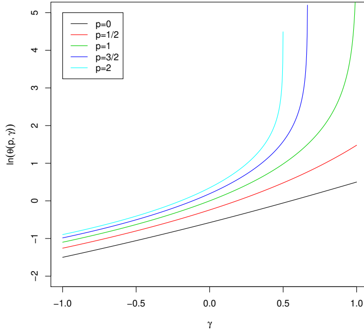
Figure 1: Graph of \gamma \mapsto \ln(\theta(p; \gamma)) for \gamma \in [-1, 1] , p \in \{0, 1/2, 1, 3/2, 2\} and under the constraint p\gamma < 1 .
