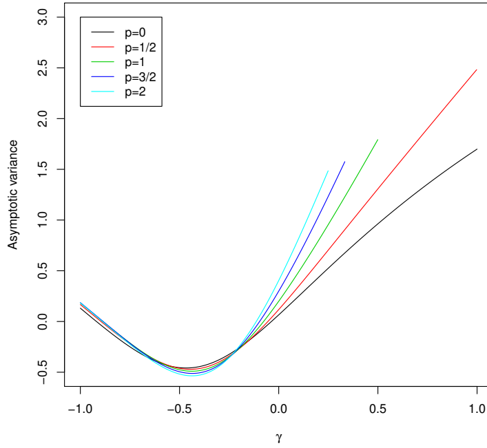
Figure 2: Graph of \gamma \mapsto \ln(\gamma^2 + 4V(p; \gamma)) for \gamma \in [-1, 1] , p \in \{0, 1/2, 1, 3/2, 2\} and under the constraint p\gamma < 1/2 .
