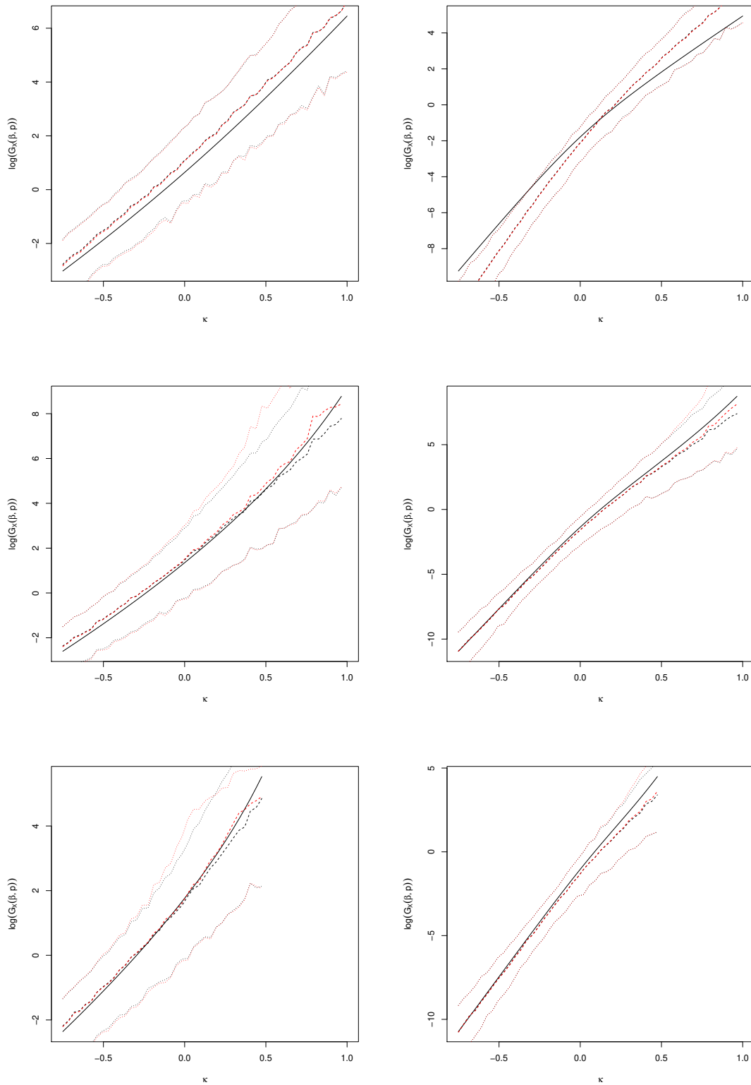
Figure 6: Simulated data, extreme case with n = 500 . The continuous line is the graph of the function \kappa \mapsto \ln G_X(\alpha_n; p) . The dashed lines represent the median of the logarithm of the N realizations of the direct (black) and indirect (red) extrapolated estimators. Dotted lines are the corresponding empirical quantiles of levels 5% and 95%. Top: p = 0 , center: p = 1 , bottom: p = 2 . Left: c = 1/2 , right: c = 2 .
