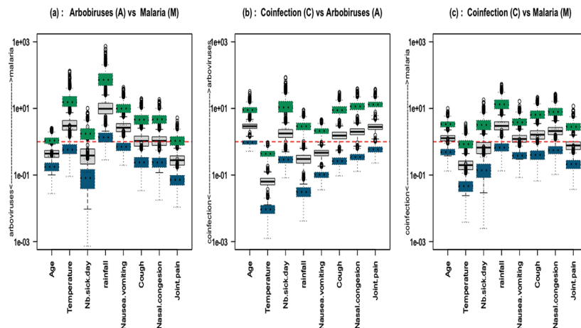
Figure 5: IgM data: boxplots of 1000 odds ratios between two categories (grey full line boxplot); boxplots of the associated confidence intervals are shown in dotted line (green for upper and blue for lower bound); (a) Arbovirus vs Malaria (b) Coinfection vs Arbovirus (c) Coinfection vs Malaria.
