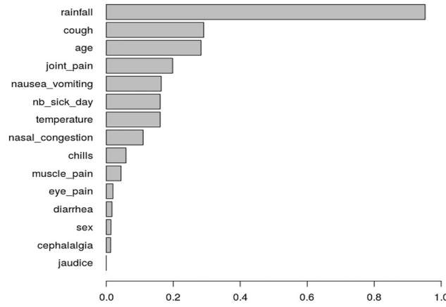
Figure 3: Ranking by VSURF: for each variable, the length of the bar corresponds to the empirical probability to be selected by VSURF among 1000 IgM sub-samples.
