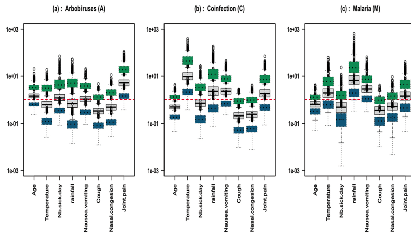
Figure 4: IgM data: boxplots of 1000 odds ratios with respect to the reference category (grey full line boxplot); boxplots of the associated confidence intervals are shown in dotted line (green for upper and blue for lower bound); (a) Arbovirus (b) Coinfection (c) Malaria.
