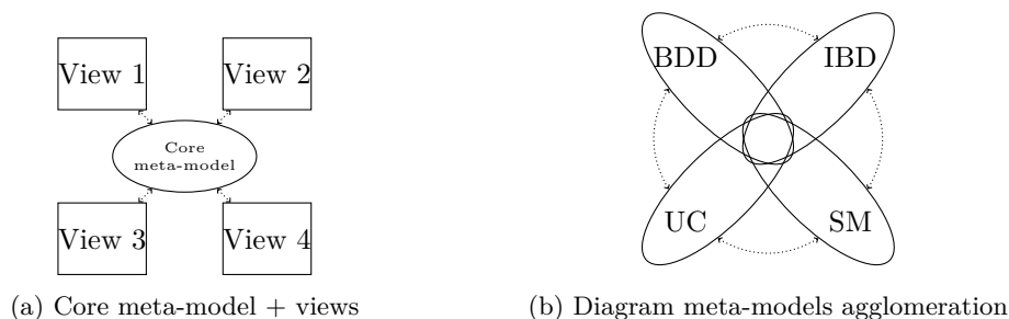
Figure 7: Metamodel structures
