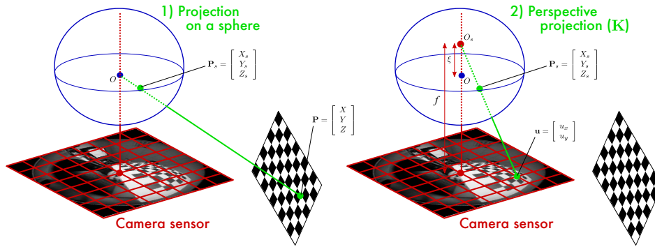
Figure 4: Unified spherical model adopted for the calibration of the camera used during our acquisition.
