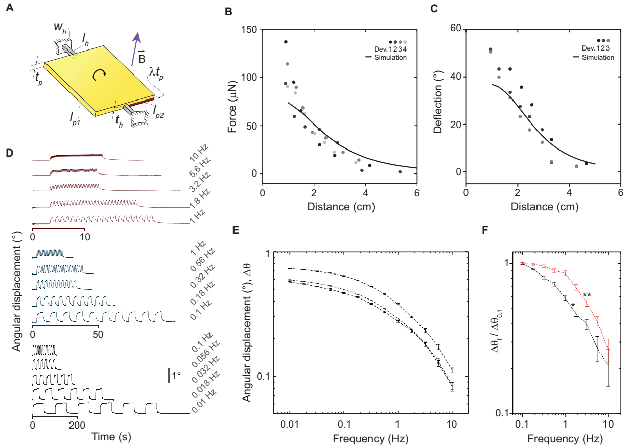
Figure 3: Actuator characteristics - forces, displacements and actuation bandwidth. (A) In order to characterize the actuator performance, we use the fundamental design (Fig. 2G) with a small change. Here only a fraction of the panel thickness, t_p , is filled with MPC, denoted by \lambda . The following results were obtained with a rectangular panel of size l_{p1} \times l_{p2} = 8 \text{ mm} \times 9 \text{ mm} , thickness t_p = 1 \text{ mm} , \lambda = 0.15 , and hinges with dimensions W_h = 0.5 \text{ mm} , l_h = 1 \text{ mm} and t_h = 0.25 \text{ mm} . (B) Measured blocking forces of 4 identical devices shown as a function of the distance from the 2'' \times 2'' \times 0.5'' magnet along with corresponding simulation results (see magnet, measurement setup and simulation details in Materials and Methods). (C) Measured angular deflections of 3 identical devices as a function of distance from the magnet. (D) Optically tracked angular displacements as function of time for actuation at frequencies from 0.01 Hz to 10 Hz. (E) Angular displacement amplitudes as a function of frequency for three devices. (F) The apparent large-amplitude bandwidth depends on the setup of the magnetic field since the force experienced by the actuator itself varies with the displacement. This is highlighted in this plot with two cases - in one case, the force experienced by the actuator increases monotonically with angular displacement ( \star ) and in the other case with a stable angular displacement when the panel aligns with the direction of maximum gradient ( \star\star ). See fig. S5 for corresponding time curves, and details of the setup.
