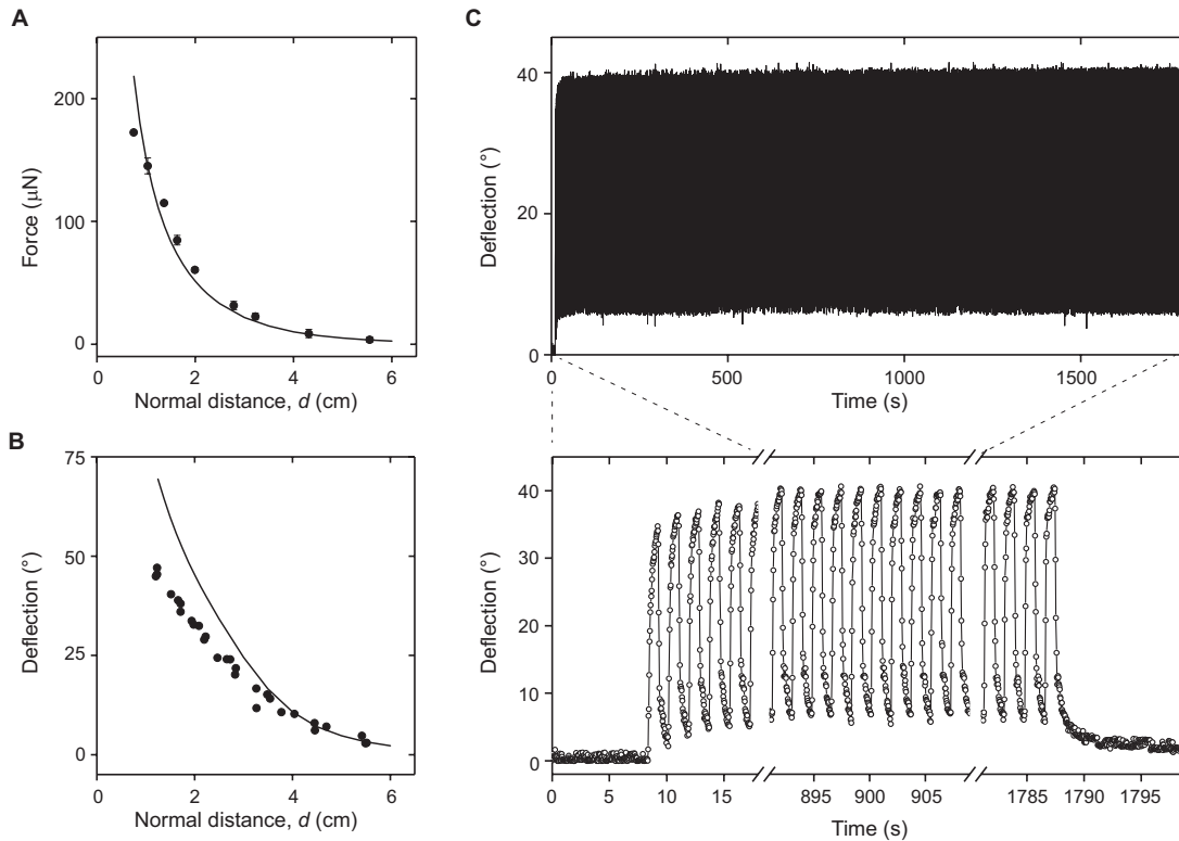
Figure 7: Characteristics of the topology-optimized actuator and long-term tests. (A) The blocking force produced by the Van Gogh actuator (Fig. 6) was measured and simulated as function of distance to the magnet. To ensure that the actuator was consistently actuated on the same side each time, the actuating magnet was offset towards one half in all simulations and experimental characterization. The measurement setup is shown in fig. S12. Also note that all simulations are performed without any fitting parameters. (B) Measured and simulated angular displacement of the topology-optimized Van Gogh actuator as a function of the normal distance between the actuator and the magnet (setup in fig. S12). (C) In order to test the long-term performance of the large actuator and the reliability of the hinges, we cycled a scaled version of the basic design (Fig. 3A) with dimensions identical to the Van Gogh actuator for 1000 cycles (see Video S3).
