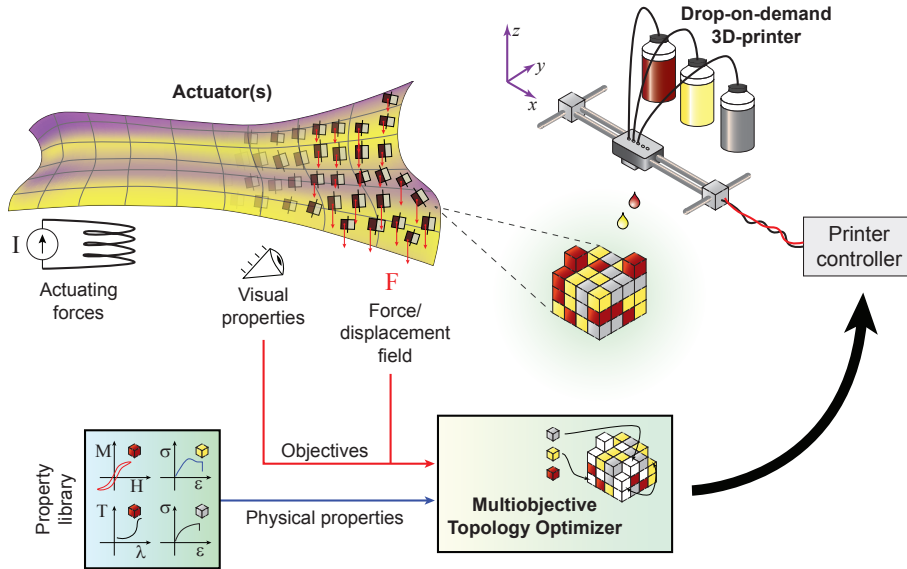
Figure 1: Overview of the specification-driven 3D-printing process. The structure of individual actuators (or the arrangement of multiple actuators) is optimized using a multi-objective topology optimization process. Note that in general, the final optimized structure can be of any arbitrary shape as shown. The optimization uses the bulk physical properties of the individual materials and the functional objectives as inputs. The generated optimized voxel-based representation of the structure is used by the printer to fabricate the optimized structure using a drop-on-demand inkjet printing process. This allows high-dimensional designs to be automatically generated and fabricated with minimal human intervention. In this work, a rigid acrylate polymer (RIG), an elastic acrylate polymer (ELA) and a magnetic nanoparticle ( \text{Fe}_3\text{O}_4 )/polymer composite (MPC) are the main materials used. The contrast in the optical, mechanical and magnetic properties is used to simultaneously optimize the visual appearance and the actuating forces while generating the voxel-level design.
