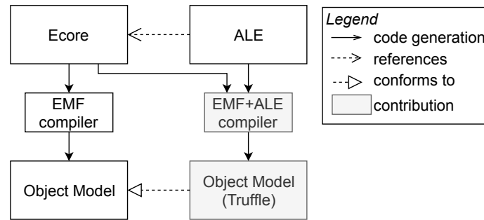
Figure 3 – Presentation of EMF’s compiler and our compiler.
