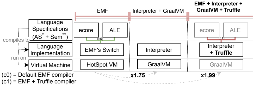
Figure 2 – General overview of the proposed approach. Decimal numbers prefixed with an x represent performance speedups. * Abstract Syntax. ** Semantics.
